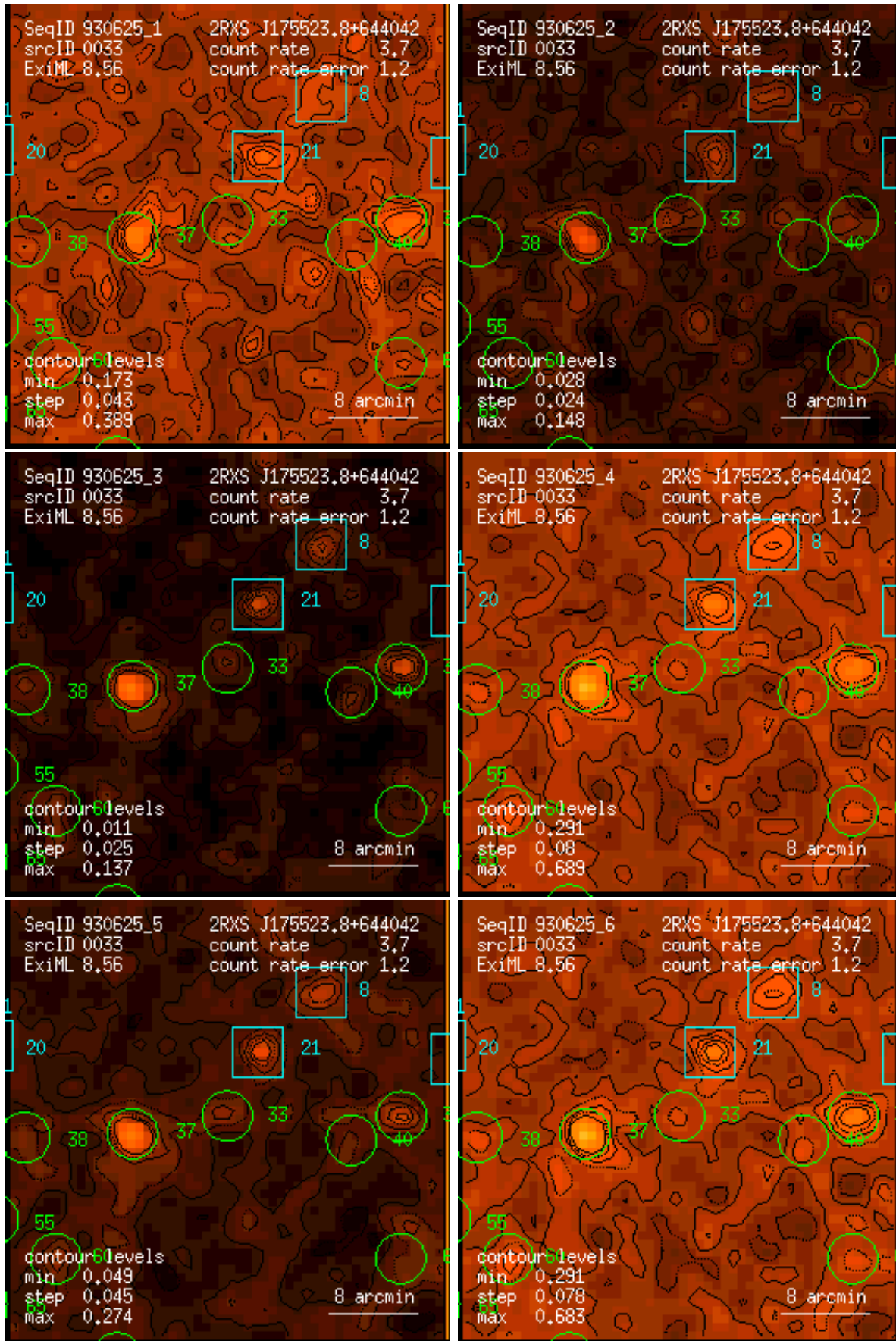
Figure 33: RASS 930625: detection 0033: band rate images, Gaussian filter: (1) PSPC channels 11 – 41, (2) 52 – 90, (3) 91 – 201, (4) 11 – 235, (5) 52 – 201, (6) 11 – 201. Broad band rates in counts/ks. Band rate contour levels in counts/ks/arcmin 2 .
