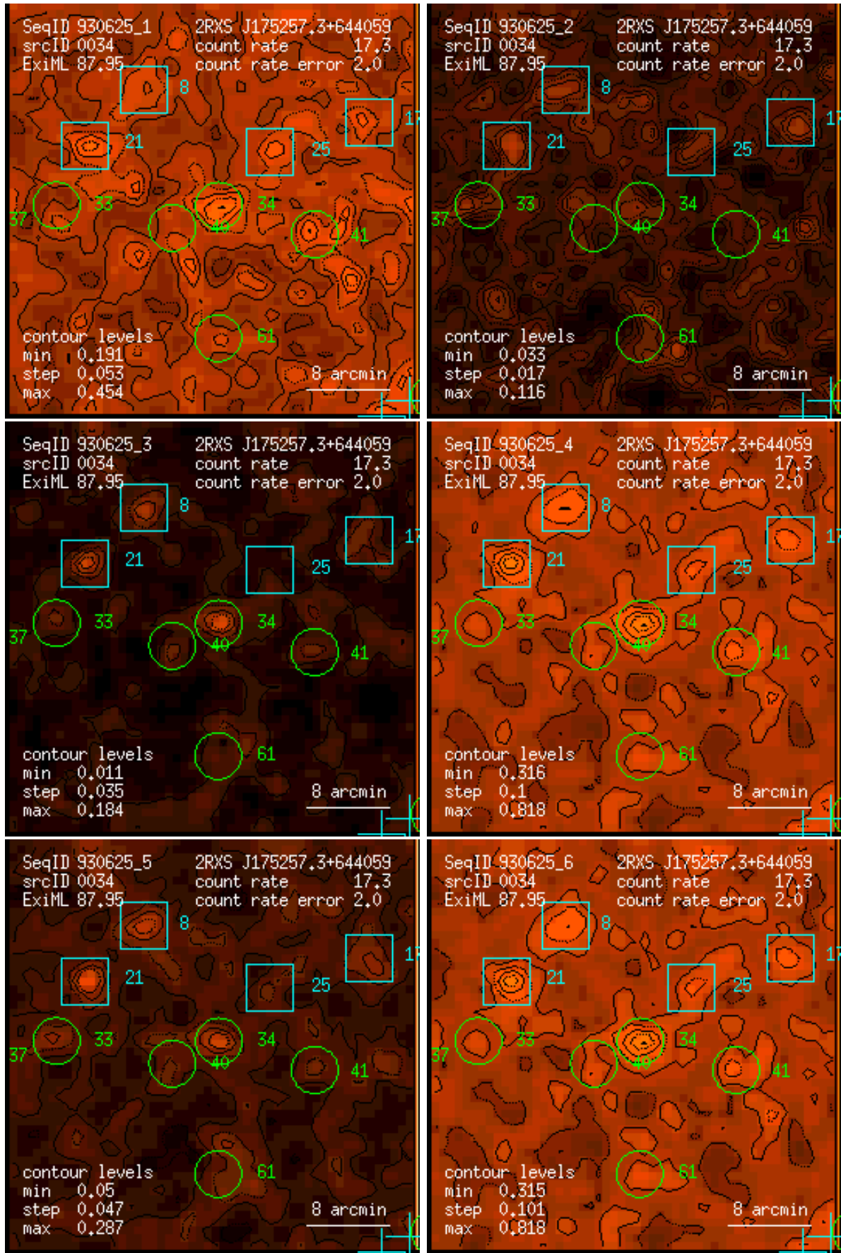
Figure 34: RASS 930625: detection 0034: band rate images, Gaussian filter: (1) PSPC channels 11 – 41, (2) 52 – 90, (3) 91 – 201, (4) 11 – 235, (5) 52 – 201, (6) 11 – 201. Broad band rates in counts/ks. Band rate contour levels in counts/ks/arcmin 2 .
