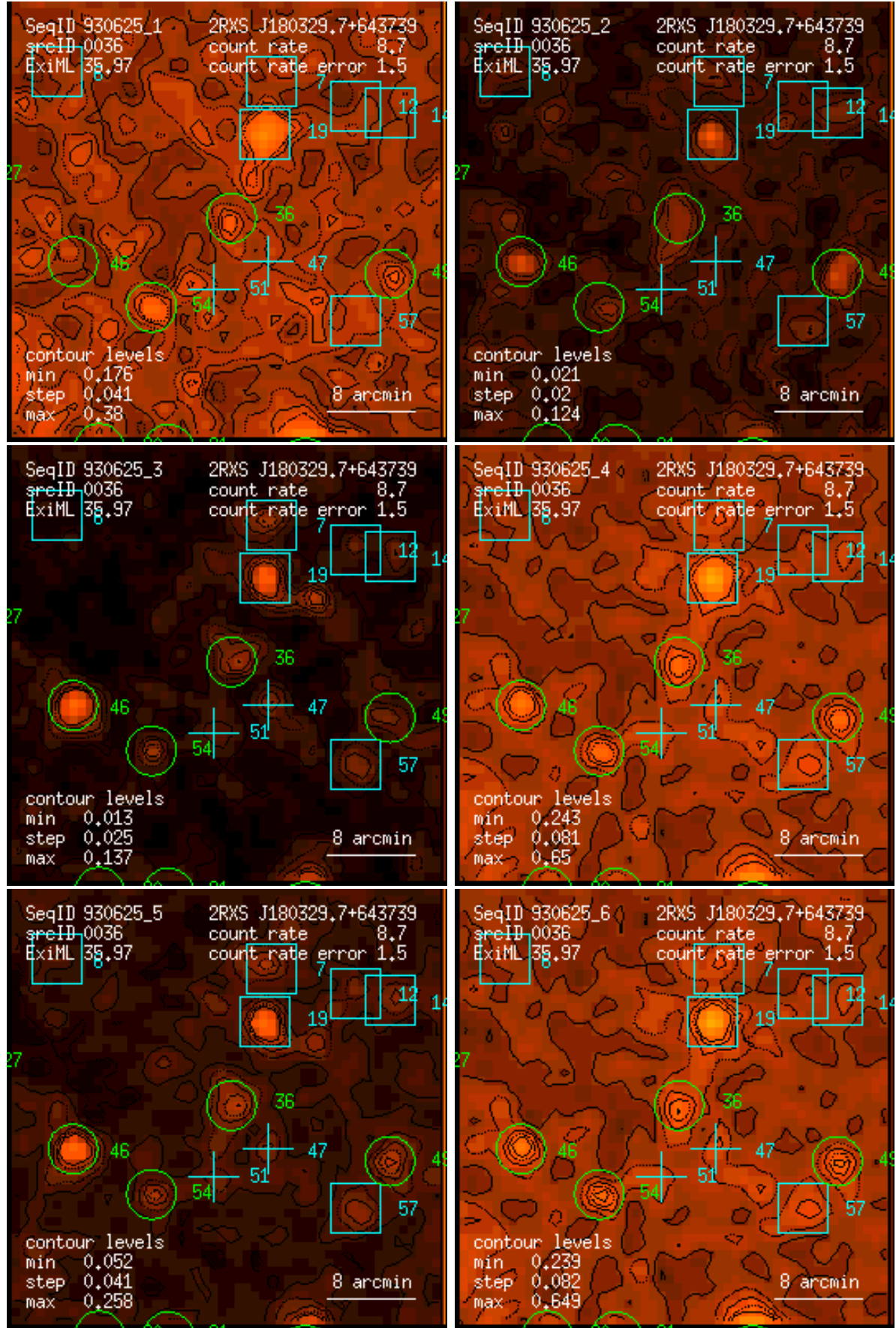
Figure 36: RASS 930625: detection 0036: band rate images, Gaussian filter: (1) PSPC channels 11 – 41, (2) 52 – 90, (3) 91 – 201, (4) 11 – 235, (5) 52 – 201, (6) 11 – 201. Broad band rates in counts/ks. Band rate contour levels in counts/ks/arcmin 2 .
