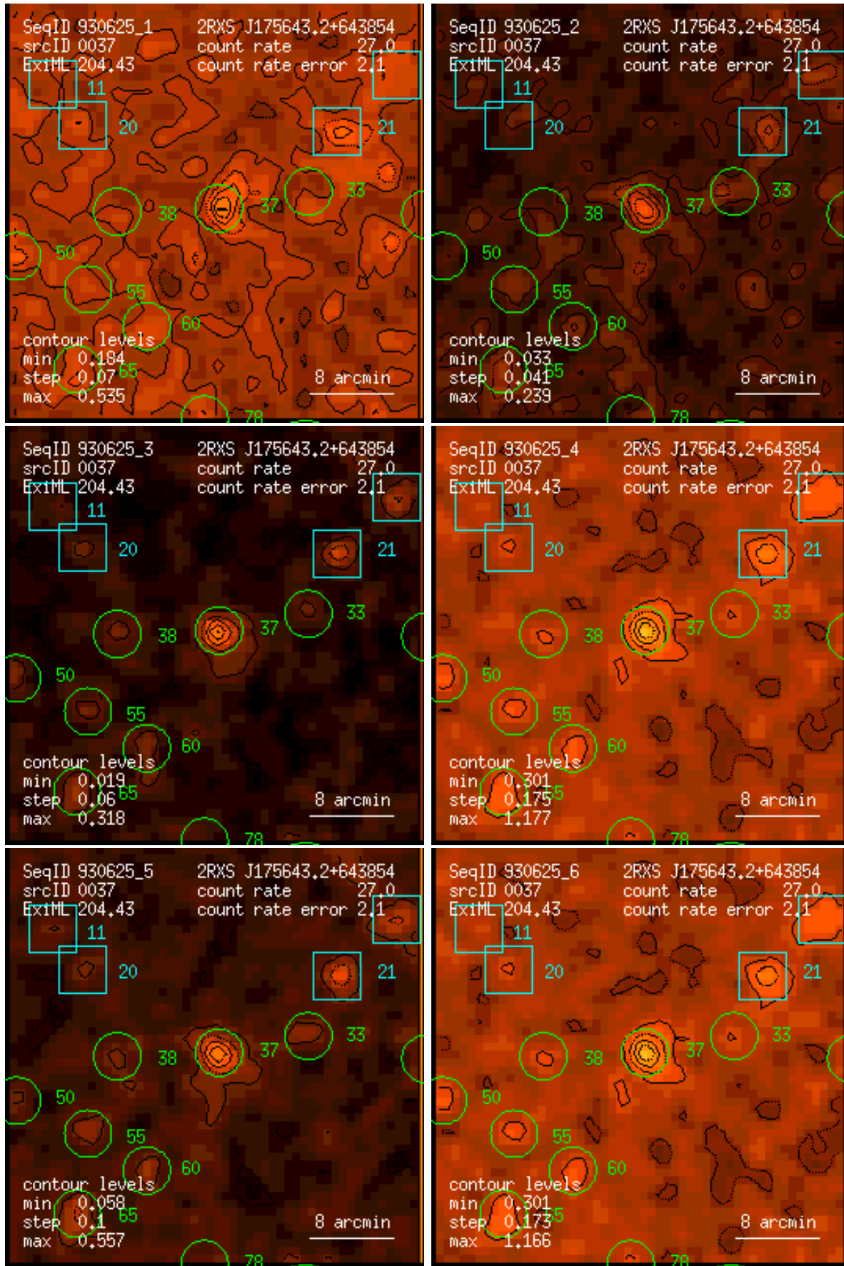
Figure 37: RASS 930625: detection 0037: band rate images, Gaussian filter: (1) PSPC channels 11 – 41, (2) 52 – 90, (3) 91 – 201, (4) 11 – 235, (5) 52 – 201, (6) 11 – 201. Broad band rates in counts/ks. Band rate contour levels in counts/ks/arcmin 2 .
