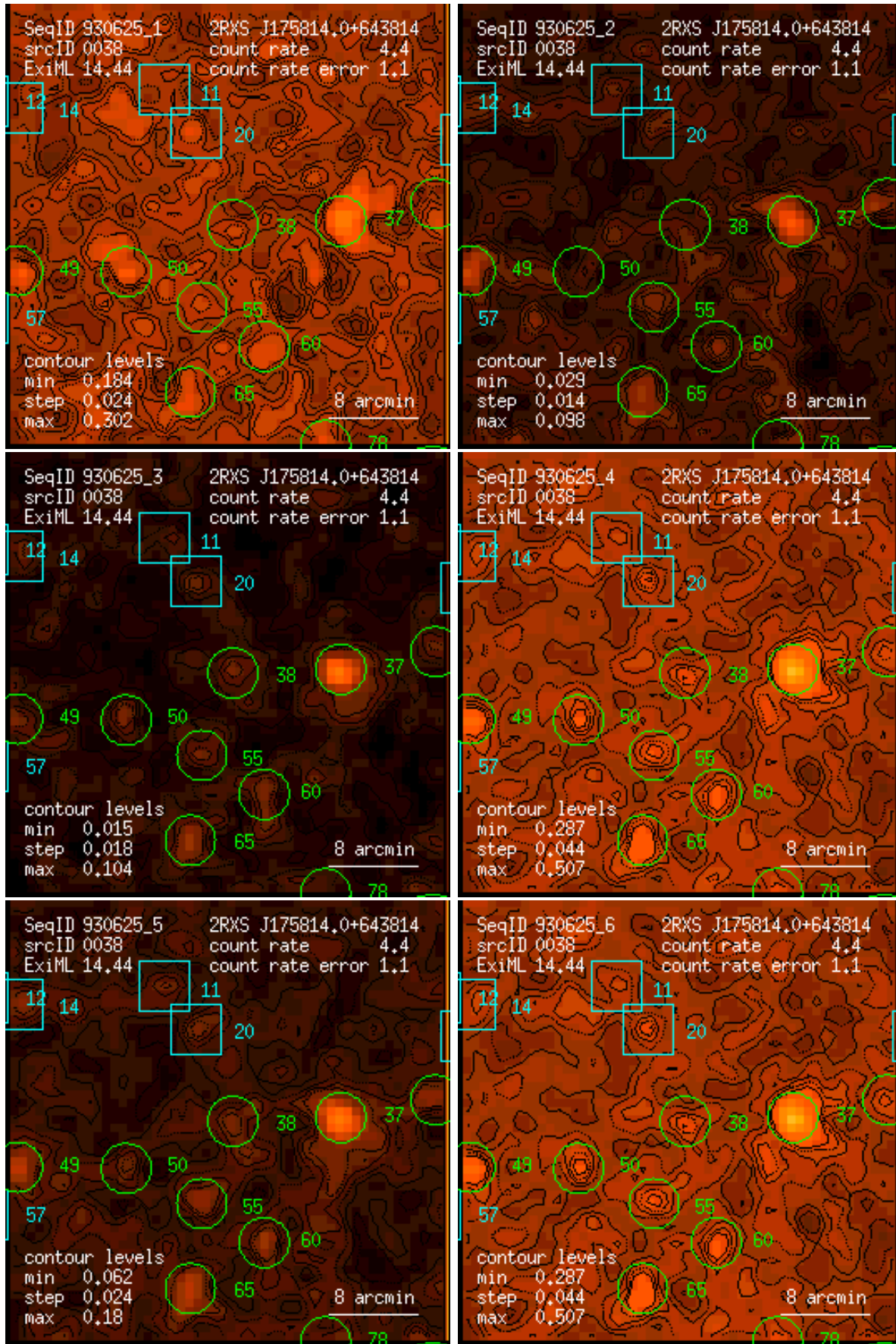
Figure 38: RASS 930625: detection 0038: band rate images, Gaussian filter: (1) PSPC channels 11 – 41, (2) 52 – 90, (3) 91 – 201, (4) 11 – 235, (5) 52 – 201, (6) 11 – 201. Broad band rates in counts/ks. Band rate contour levels in counts/ks/arcmin 2 .
