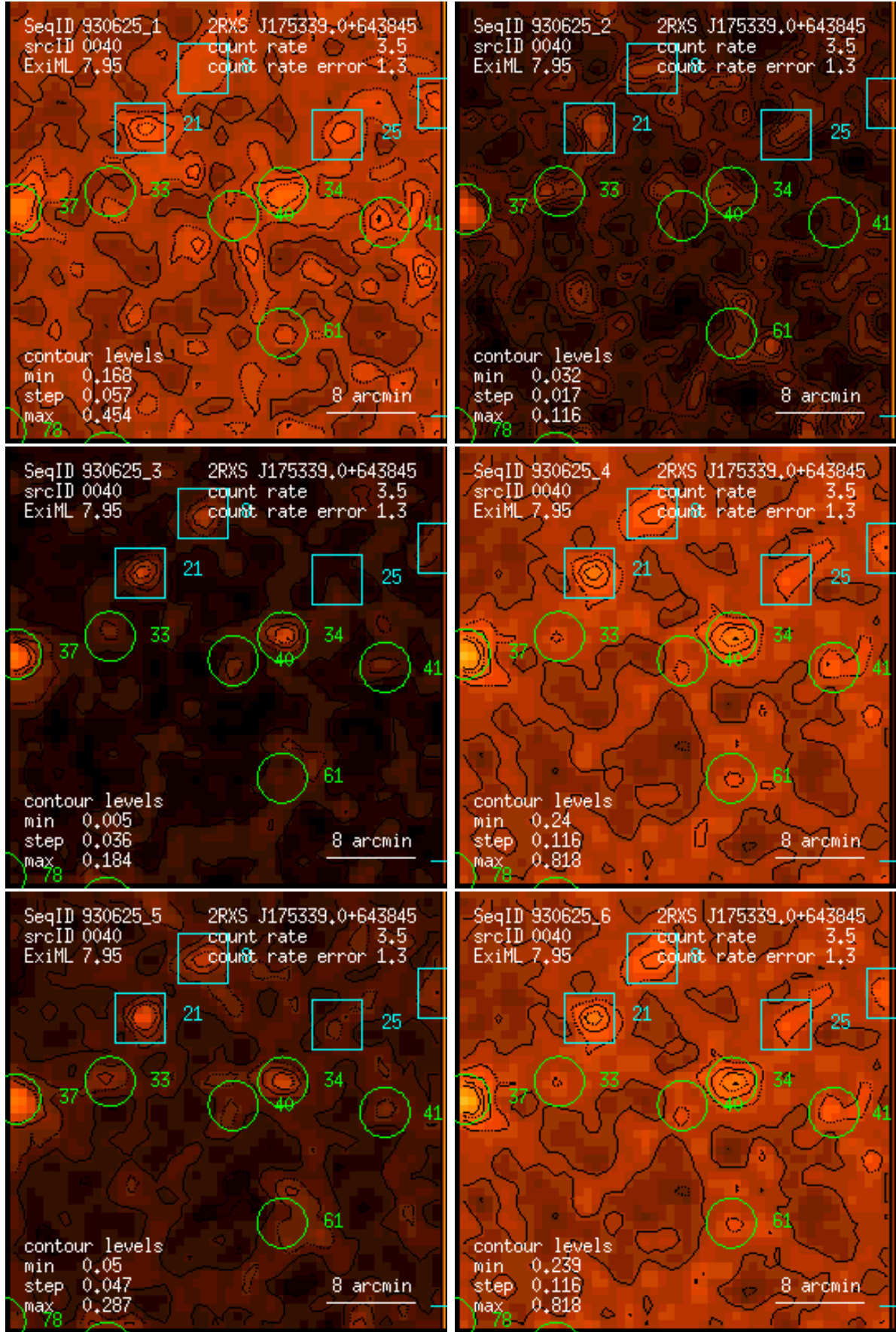
Figure 40: RASS 930625: detection 0040: band rate images, Gaussian filter: (1) PSPC channels 11 – 41, (2) 52 – 90, (3) 91 – 201, (4) 11 – 235, (5) 52 – 201, (6) 11 – 201. Broad band rates in counts/ks. Band rate contour levels in counts/ks/arcmin 2 .
