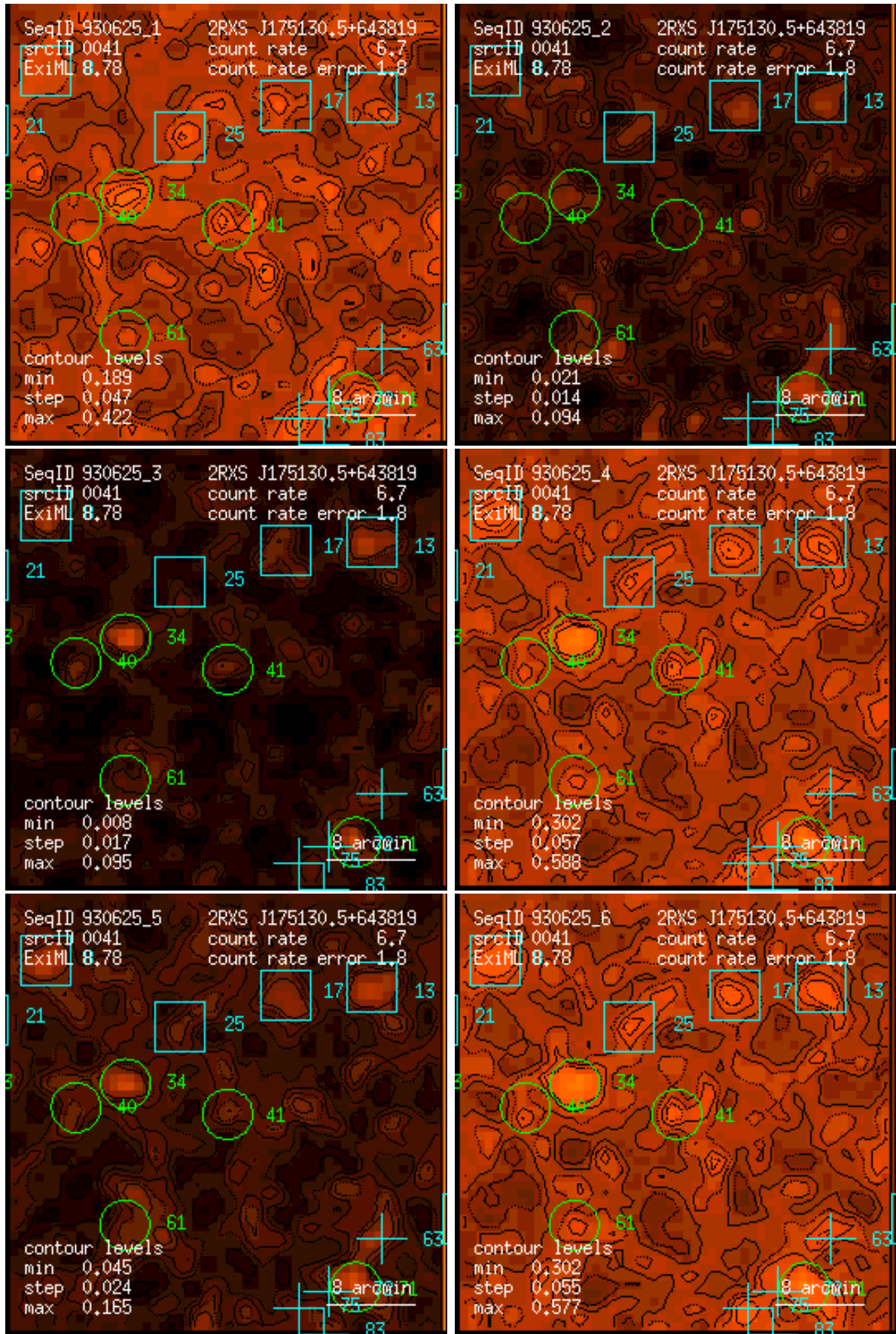
Figure 41: RASS 930625: detection 0041: band rate images, Gaussian filter: (1) PSPC channels 11 – 41, (2) 52 – 90, (3) 91 – 201, (4) 11 – 235, (5) 52 – 201, (6) 11 – 201. Broad band rates in counts/ks. Band rate contour levels in counts/ks/arcmin 2 .
