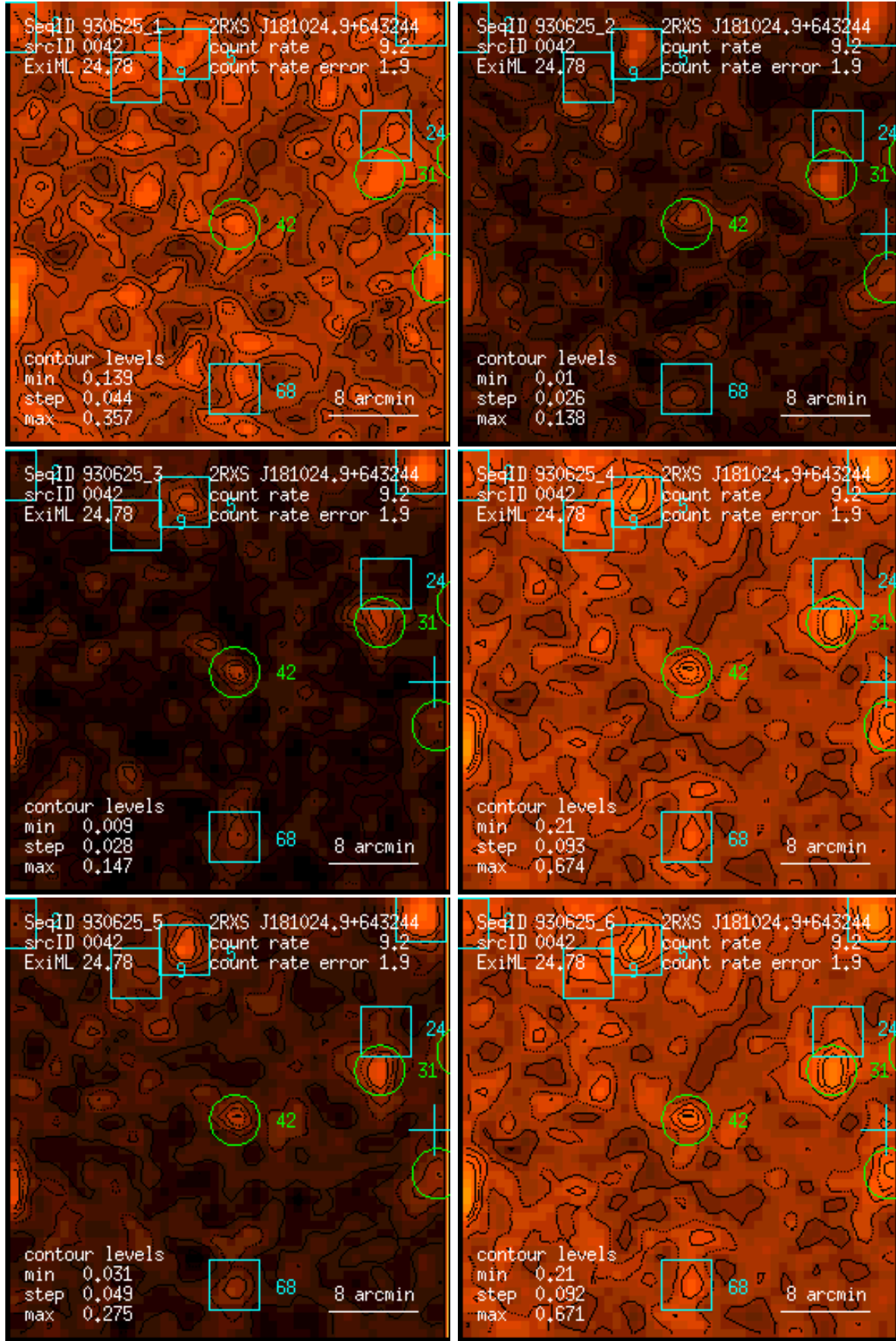
Figure 42: RASS 930625: detection 0042: band rate images, Gaussian filter: (1) PSPC channels 11 – 41, (2) 52 – 90, (3) 91 – 201, (4) 11 – 235, (5) 52 – 201, (6) 11 – 201. Broad band rates in counts/ks. Band rate contour levels in counts/ks/arcmin 2 .
