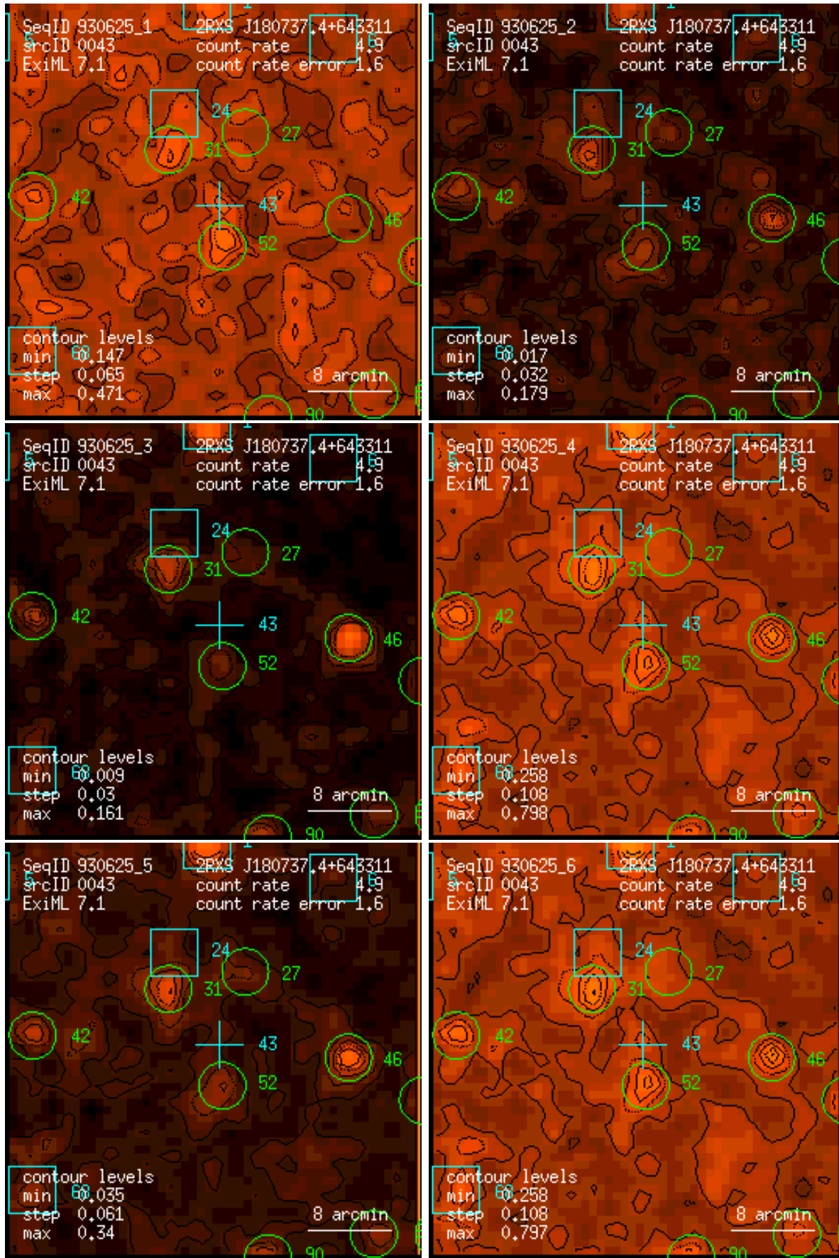
Figure 43: RASS 930625: detection 0043: band rate images, Gaussian filter: (1) PSPC channels 11 – 41, (2) 52 – 90, (3) 91 – 201, (4) 11 – 235, (5) 52 – 201, (6) 11 – 201. Broad band rates in counts/ks. Band rate contour levels in counts/ks/arcmin 2 .
