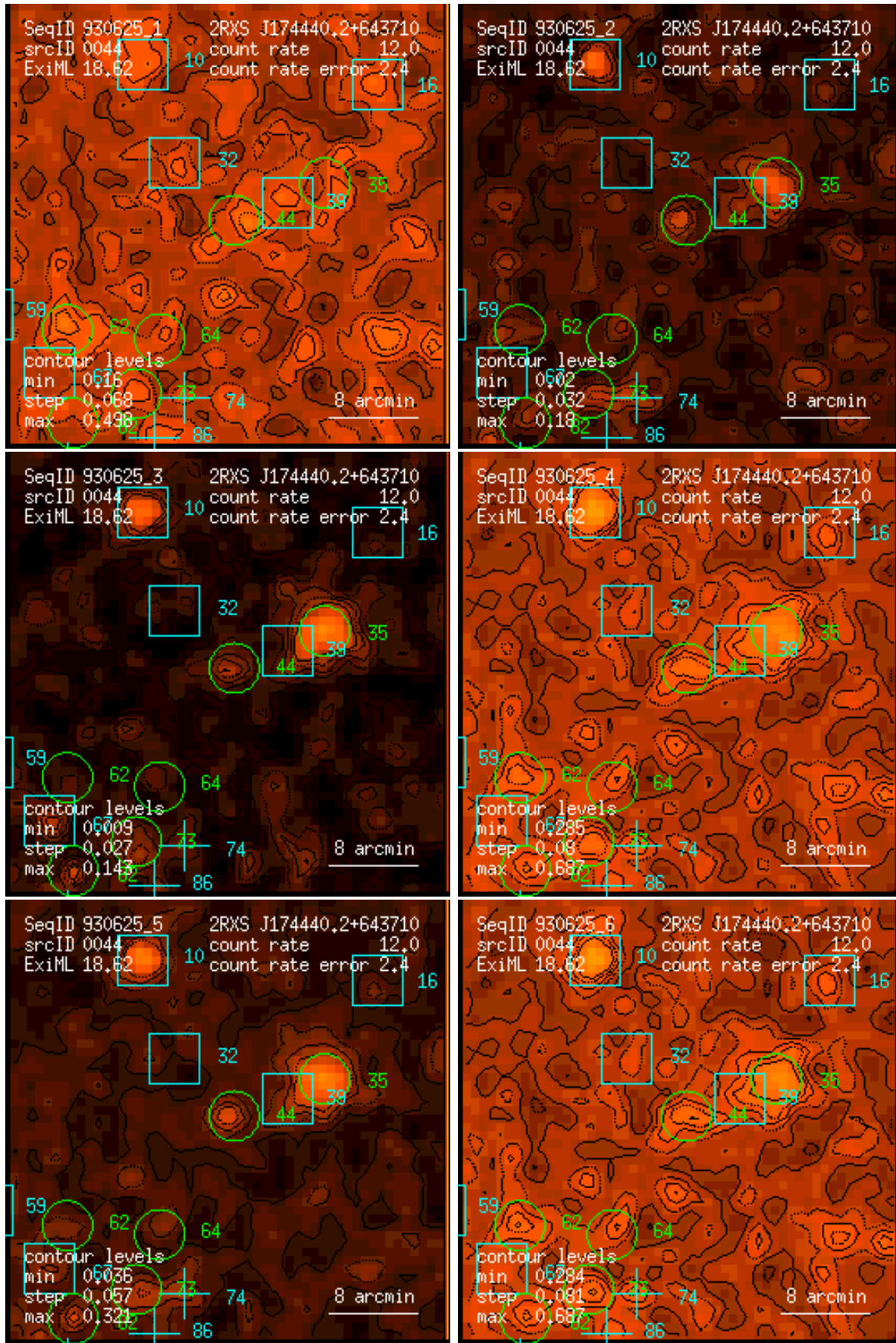
Figure 44: RASS 930625: detection 0044: band rate images, Gaussian filter: (1) PSPC channels 11 – 41, (2) 52 – 90, (3) 91 – 201, (4) 11 – 235, (5) 52 – 201, (6) 11 – 201. Broad band rates in counts/ks. Band rate contour levels in counts/ks/arcmin 2 .
