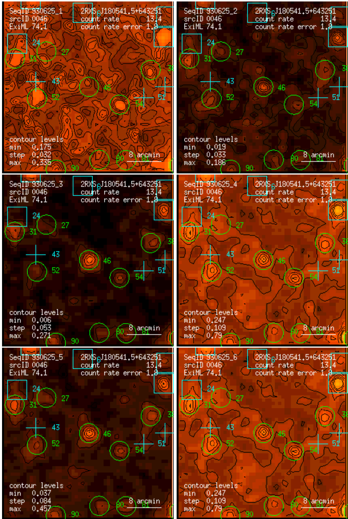
Figure 46: RASS 930625: detection 0046: band rate images, Gaussian filter: (1) PSPC channels 11 – 41, (2) 52 – 90, (3) 91 – 201, (4) 11 – 235, (5) 52 – 201, (6) 11 – 201. Broad band rates in counts/ks. Band rate contour levels in counts/ks/arcmin 2 .
