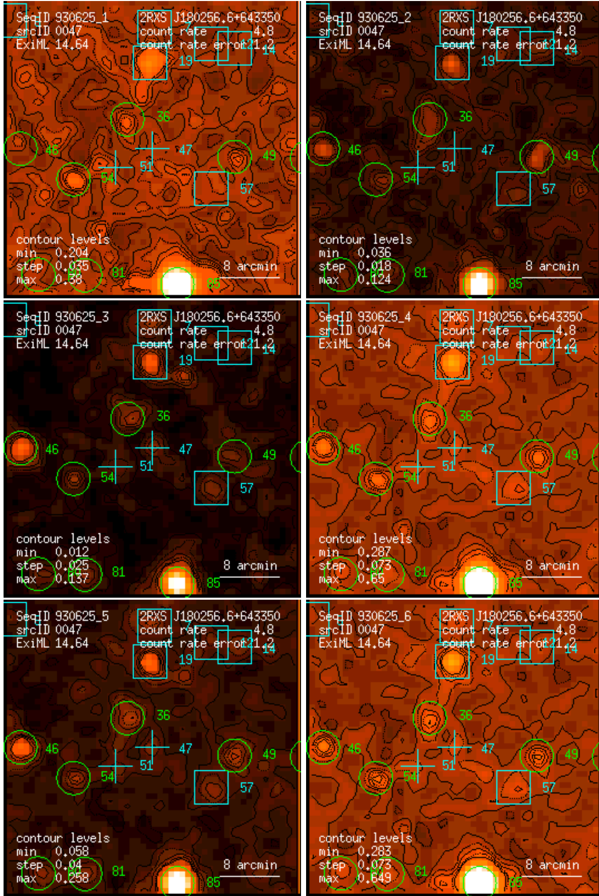
Figure 47: RASS 930625: detection 0047: band rate images, Gaussian filter: (1) PSPC channels 11 – 41, (2) 52 – 90, (3) 91 – 201, (4) 11 – 235, (5) 52 – 201, (6) 11 – 201. Broad band rates in counts/ks. Band rate contour levels in counts/ks/arcmin 2 .
