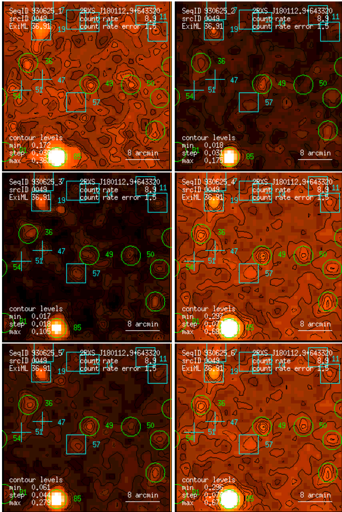
Figure 49: RASS 930625: detection 0049: band rate images, Gaussian filter: (1) PSPC channels 11 – 41, (2) 52 – 90, (3) 91 – 201, (4) 11 – 235, (5) 52 – 201, (6) 11 – 201. Broad band rates in counts/ks. Band rate contour levels in counts/ks/arcmin 2 .
