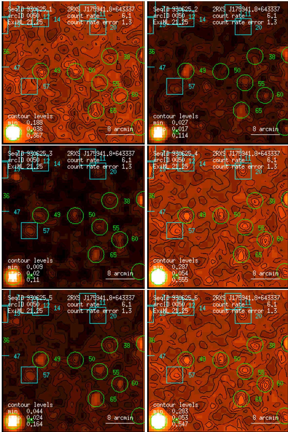
Figure 50: RASS 930625: detection 0050: band rate images, Gaussian filter: (1) PSPC channels 11 – 41, (2) 52 – 90, (3) 91 – 201, (4) 11 – 235, (5) 52 – 201, (6) 11 – 201. Broad band rates in counts/ks. Band rate contour levels in counts/ks/arcmin 2 .
