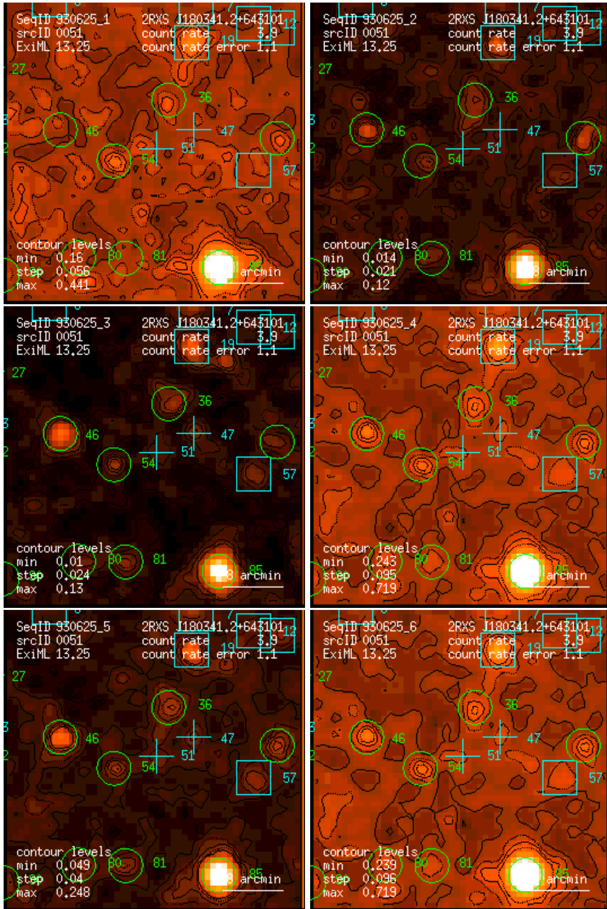
Figure 51: RASS 930625: detection 0051: band rate images, Gaussian filter: (1) PSPC channels 11 – 41, (2) 52 – 90, (3) 91 – 201, (4) 11 – 235, (5) 52 – 201, (6) 11 – 201. Broad band rates in counts/ks. Band rate contour levels in counts/ks/arcmin 2 .
