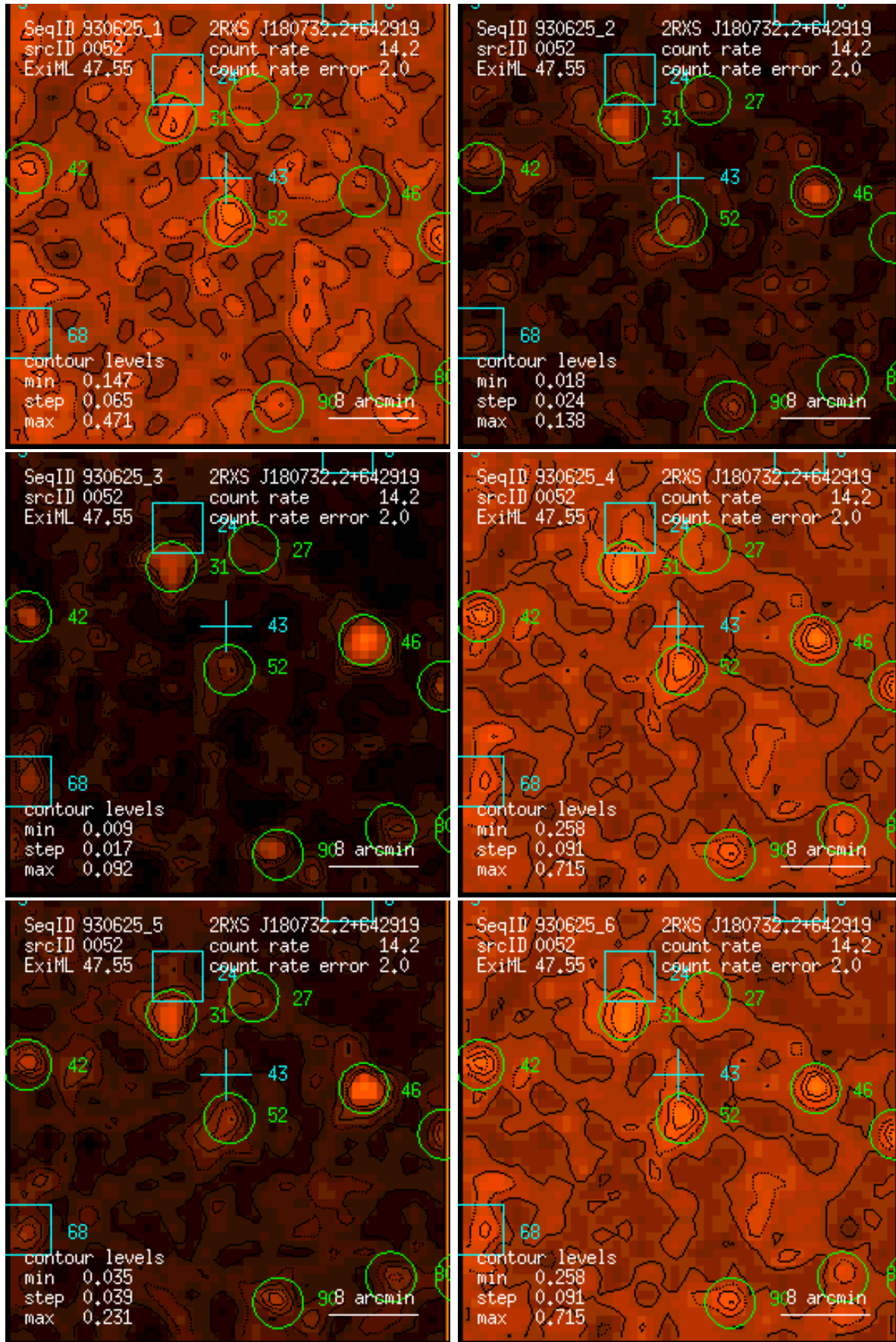
Figure 52: RASS 930625: detection 0052: band rate images, Gaussian filter: (1) PSPC channels 11 – 41, (2) 52 – 90, (3) 91 – 201, (4) 11 – 235, (5) 52 – 201, (6) 11 – 201. Broad band rates in counts/ks. Band rate contour levels in counts/ks/arcmin 2 .
