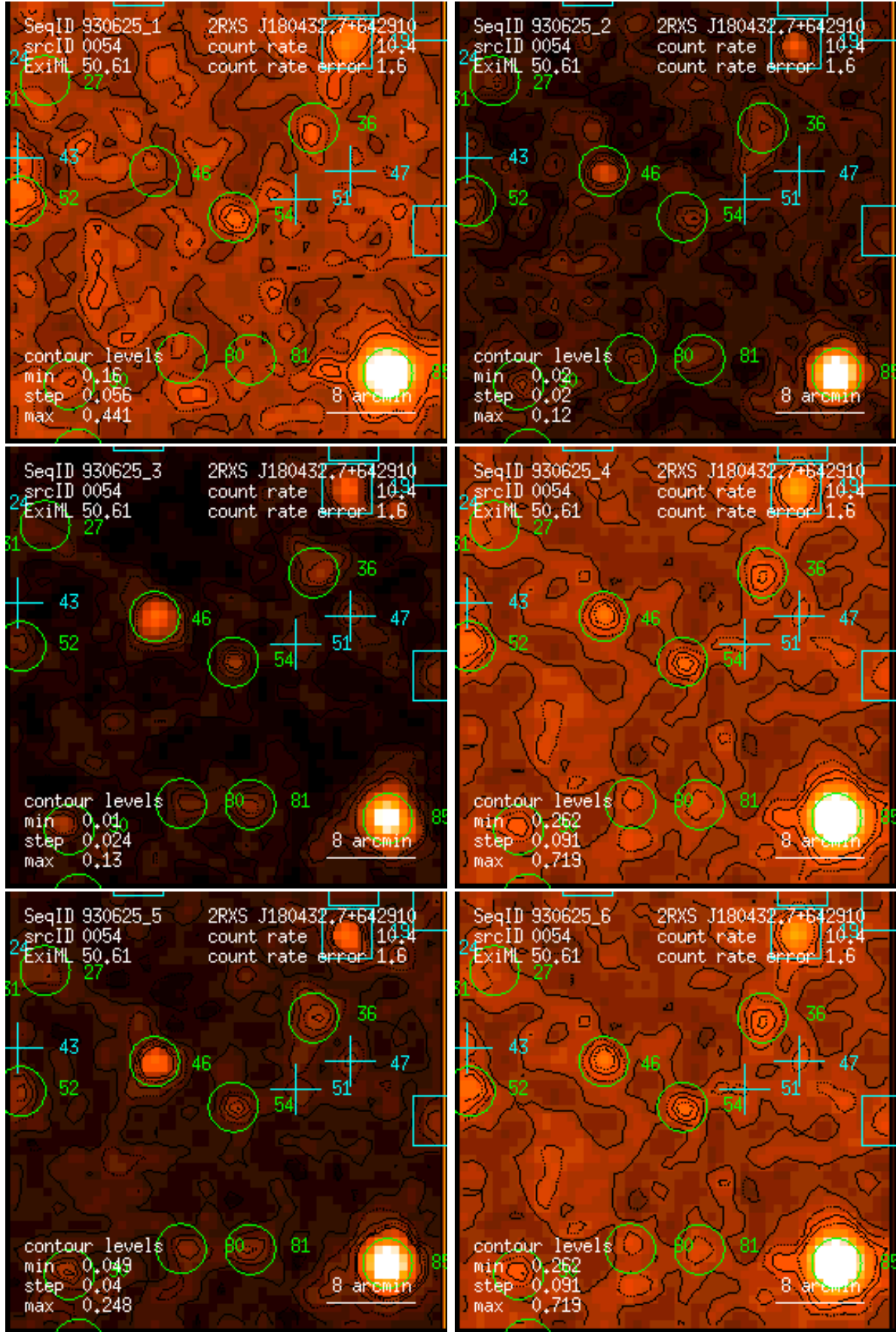
Figure 54: RASS 930625: detection 0054: band rate images, Gaussian filter: (1) PSPC channels 11 – 41, (2) 52 – 90, (3) 91 – 201, (4) 11 – 235, (5) 52 – 201, (6) 11 – 201. Broad band rates in counts/ks. Band rate contour levels in counts/ks/arcmin 2 .
