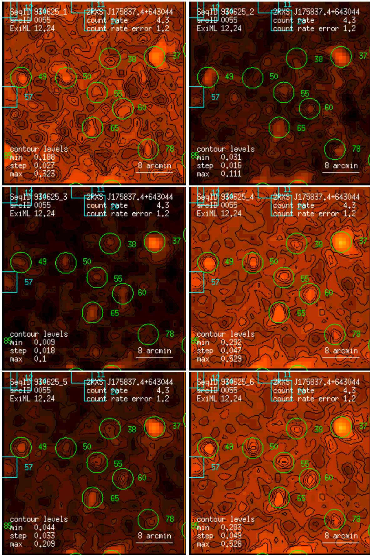
Figure 55: RASS 930625: detection 0055: band rate images, Gaussian filter: (1) PSPC channels 11 – 41, (2) 52 – 90, (3) 91 – 201, (4) 11 – 235, (5) 52 – 201, (6) 11 – 201. Broad band rates in counts/ks. Band rate contour levels in counts/ks/arcmin 2 .
