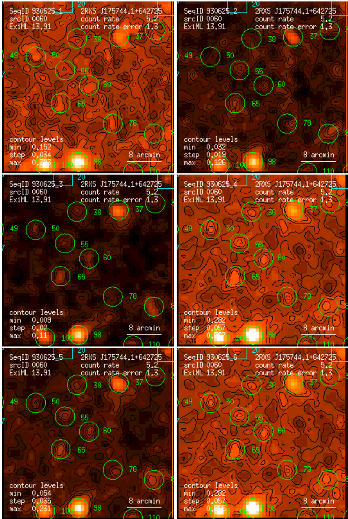
Figure 60: RASS 930625: detection 0060: band rate images, Gaussian filter: (1) PSPC channels 11 – 41, (2) 52 – 90, (3) 91 – 201, (4) 11 – 235, (5) 52 – 201, (6) 11 – 201. Broad band rates in counts/ks. Band rate contour levels in counts/ks/arcmin 2 .
