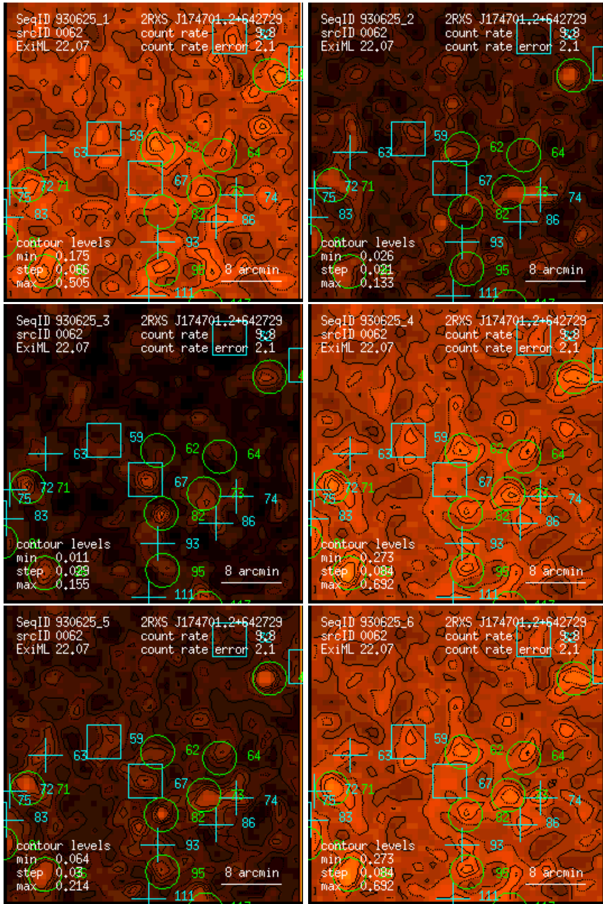
Figure 62: RASS 930625: detection 0062: band rate images, Gaussian filter: (1) PSPC channels 11 – 41, (2) 52 – 90, (3) 91 – 201, (4) 11 – 235, (5) 52 – 201, (6) 11 – 201. Broad band rates in counts/ks. Band rate contour levels in counts/ks/arcmin 2 .
