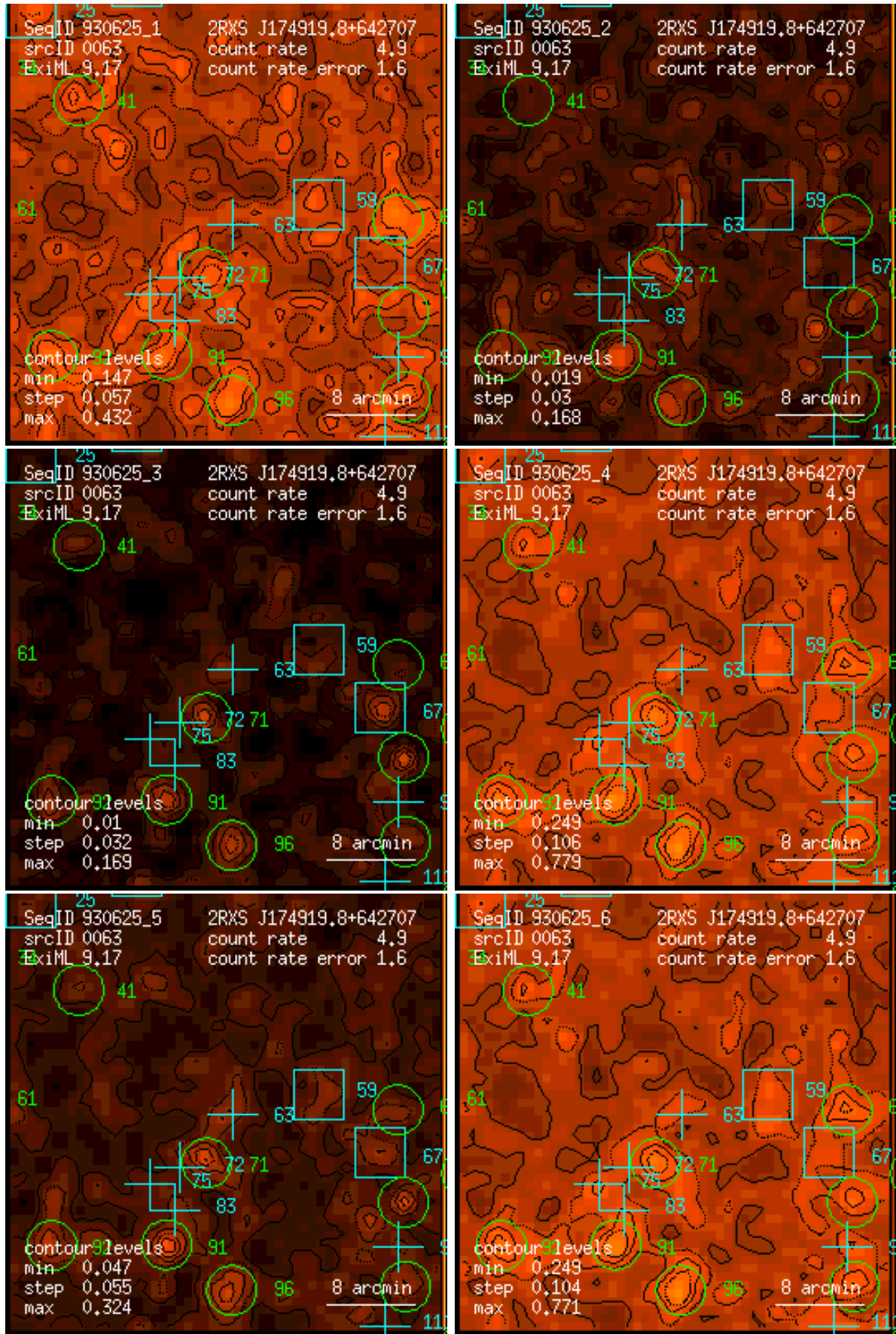
Figure 63: RASS 930625: detection 0063: band rate images, Gaussian filter: (1) PSPC channels 11 – 41, (2) 52 – 90, (3) 91 – 201, (4) 11 – 235, (5) 52 – 201, (6) 11 – 201. Broad band rates in counts/ks. Band rate contour levels in counts/ks/arcmin 2 .
