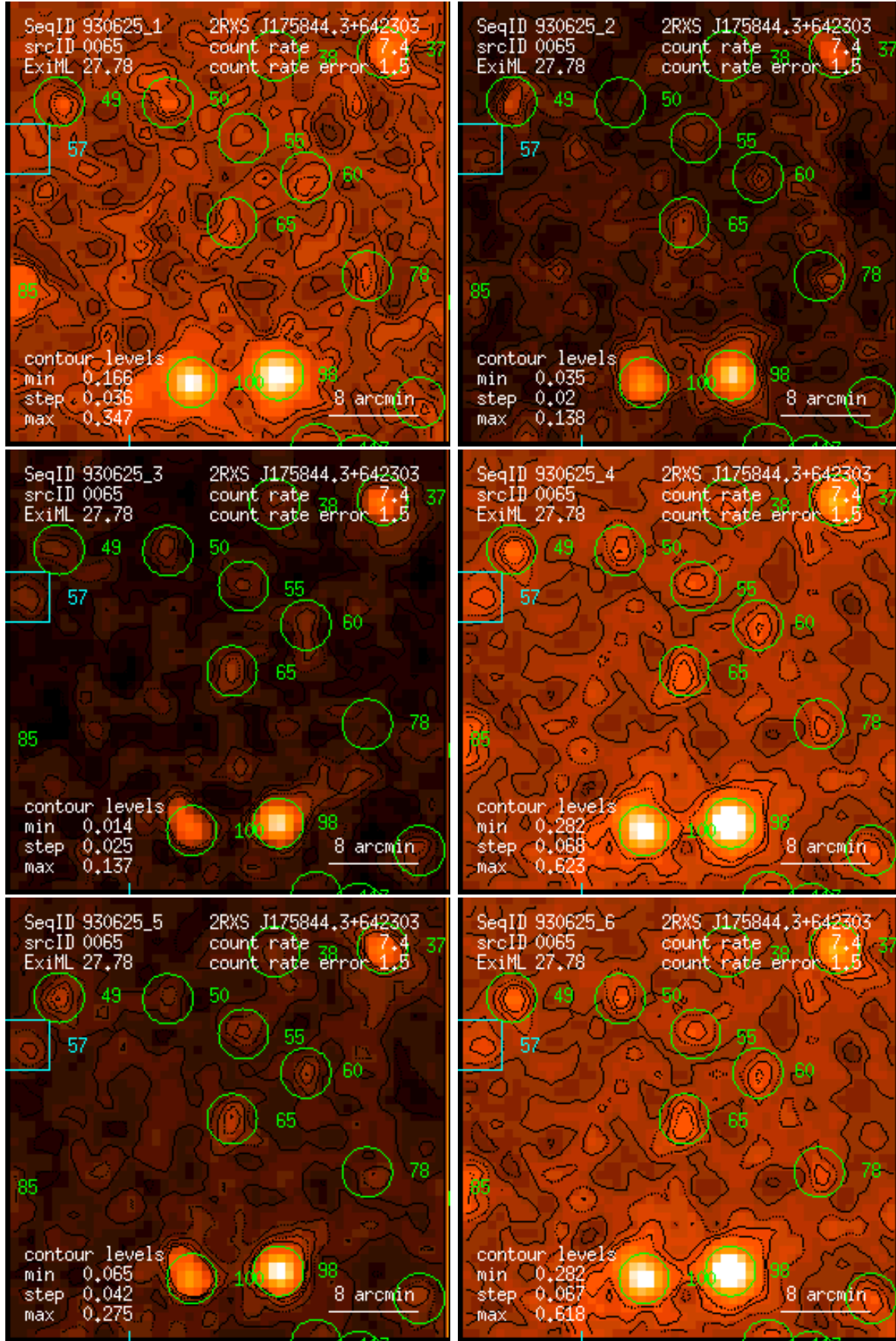
Figure 65: RASS 930625: detection 0065: band rate images, Gaussian filter: (1) PSPC channels 11 – 41, (2) 52 – 90, (3) 91 – 201, (4) 11 – 235, (5) 52 – 201, (6) 11 – 201. Broad band rates in counts/ks. Band rate contour levels in counts/ks/arcmin 2 .
