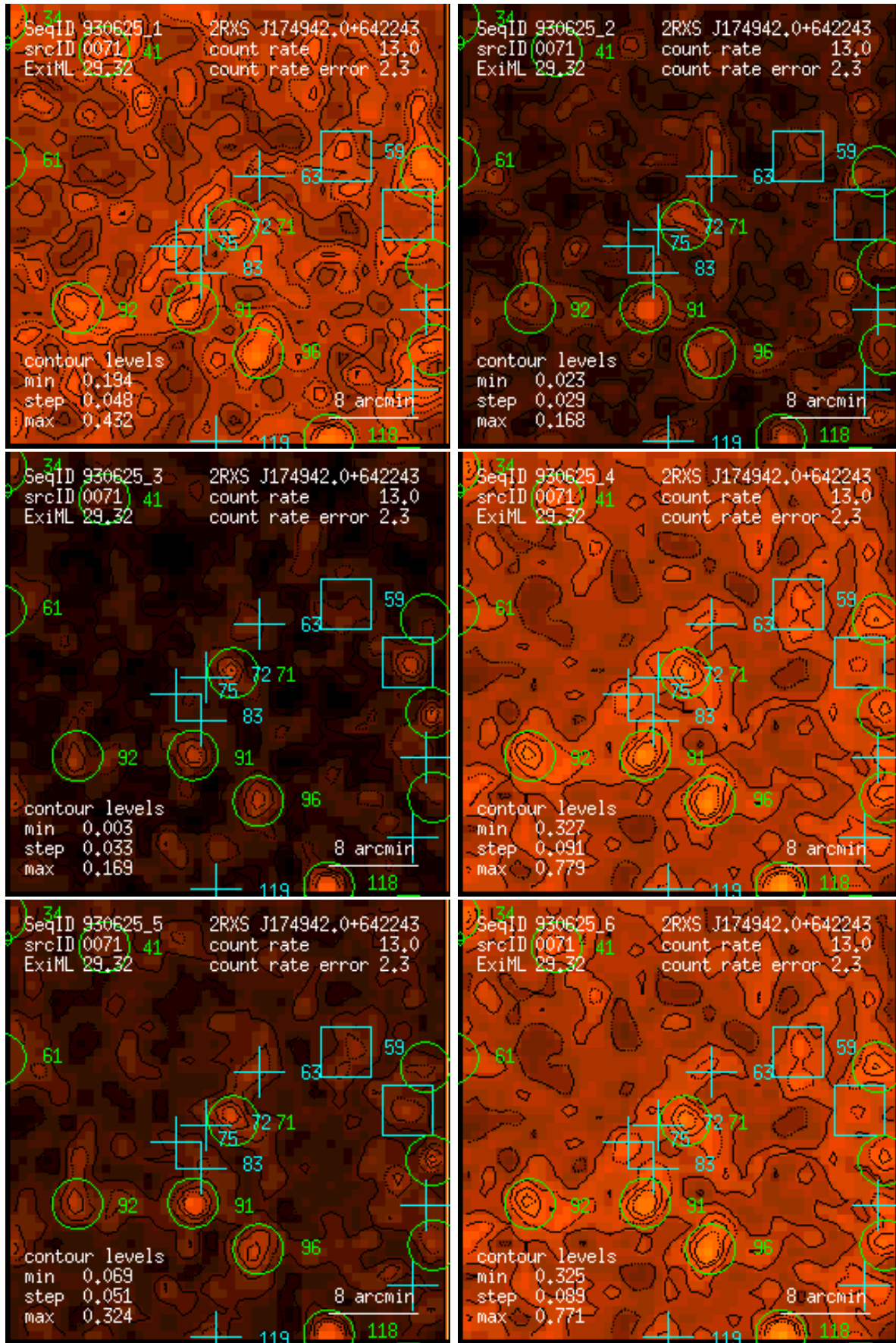
Figure 71: RASS 930625: detection 0071: band rate images, Gaussian filter: (1) PSPC channels 11 – 41, (2) 52 – 90, (3) 91 – 201, (4) 11 – 235, (5) 52 – 201, (6) 11 – 201. Broad band rates in counts/ks. Band rate contour levels in counts/ks/arcmin 2 .
