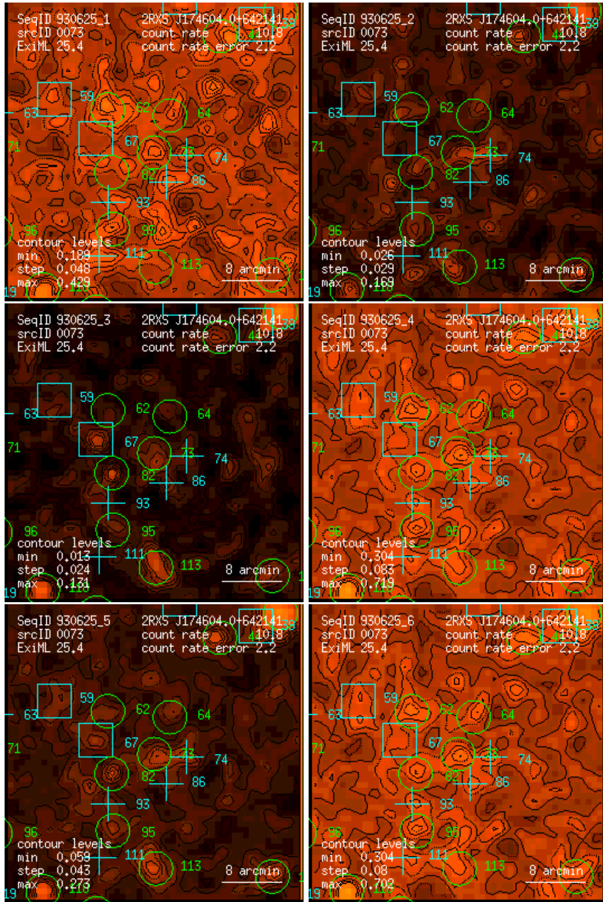
Figure 73: RASS 930625: detection 0073: band rate images, Gaussian filter: (1) PSPC channels 11 – 41, (2) 52 – 90, (3) 91 – 201, (4) 11 – 235, (5) 52 – 201, (6) 11 – 201. Broad band rates in counts/ks. Band rate contour levels in counts/ks/arcmin 2 .
