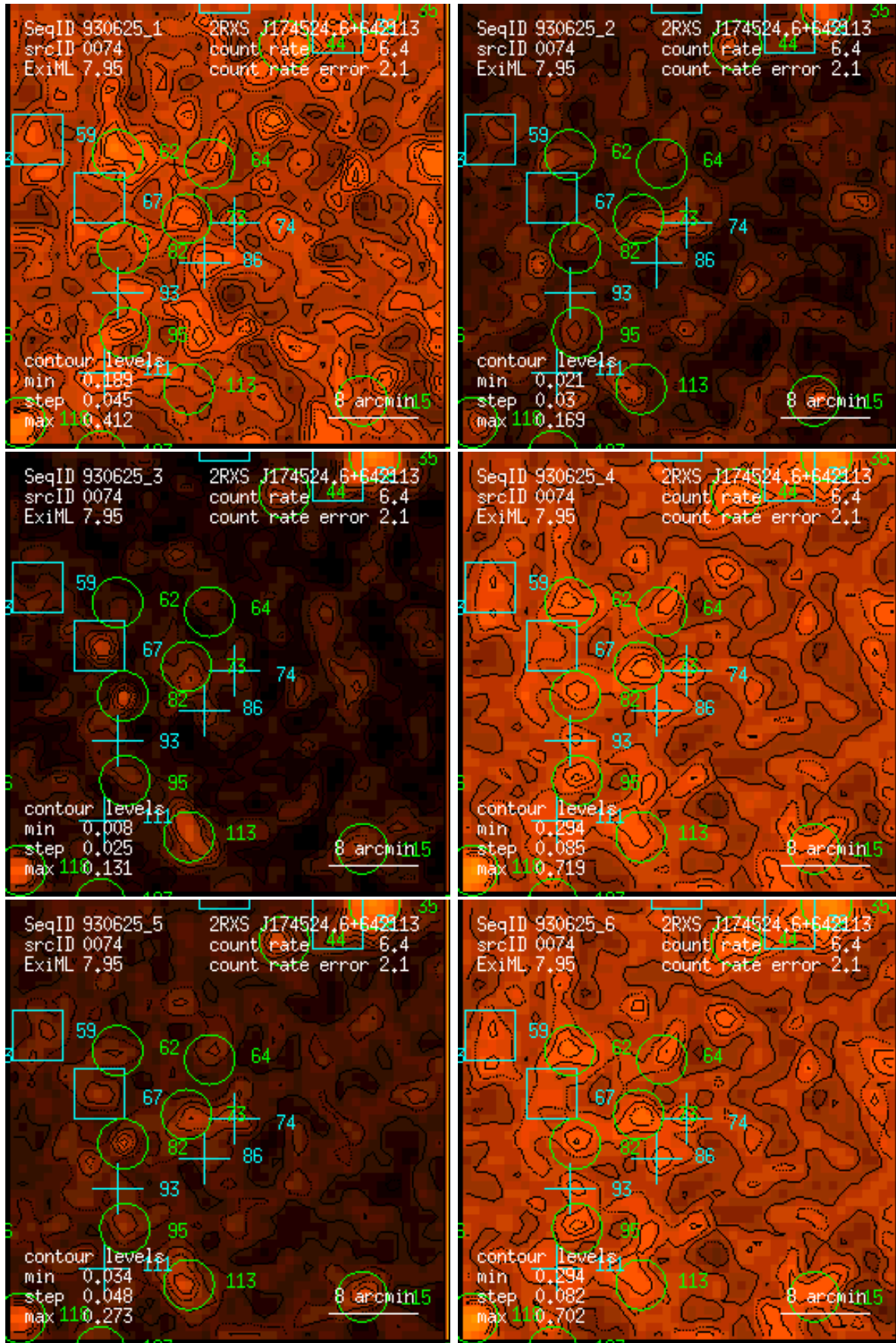
Figure 74: RASS 930625: detection 0074: band rate images, Gaussian filter: (1) PSPC channels 11 – 41, (2) 52 – 90, (3) 91 – 201, (4) 11 – 235, (5) 52 – 201, (6) 11 – 201. Broad band rates in counts/ks. Band rate contour levels in counts/ks/arcmin 2 .
