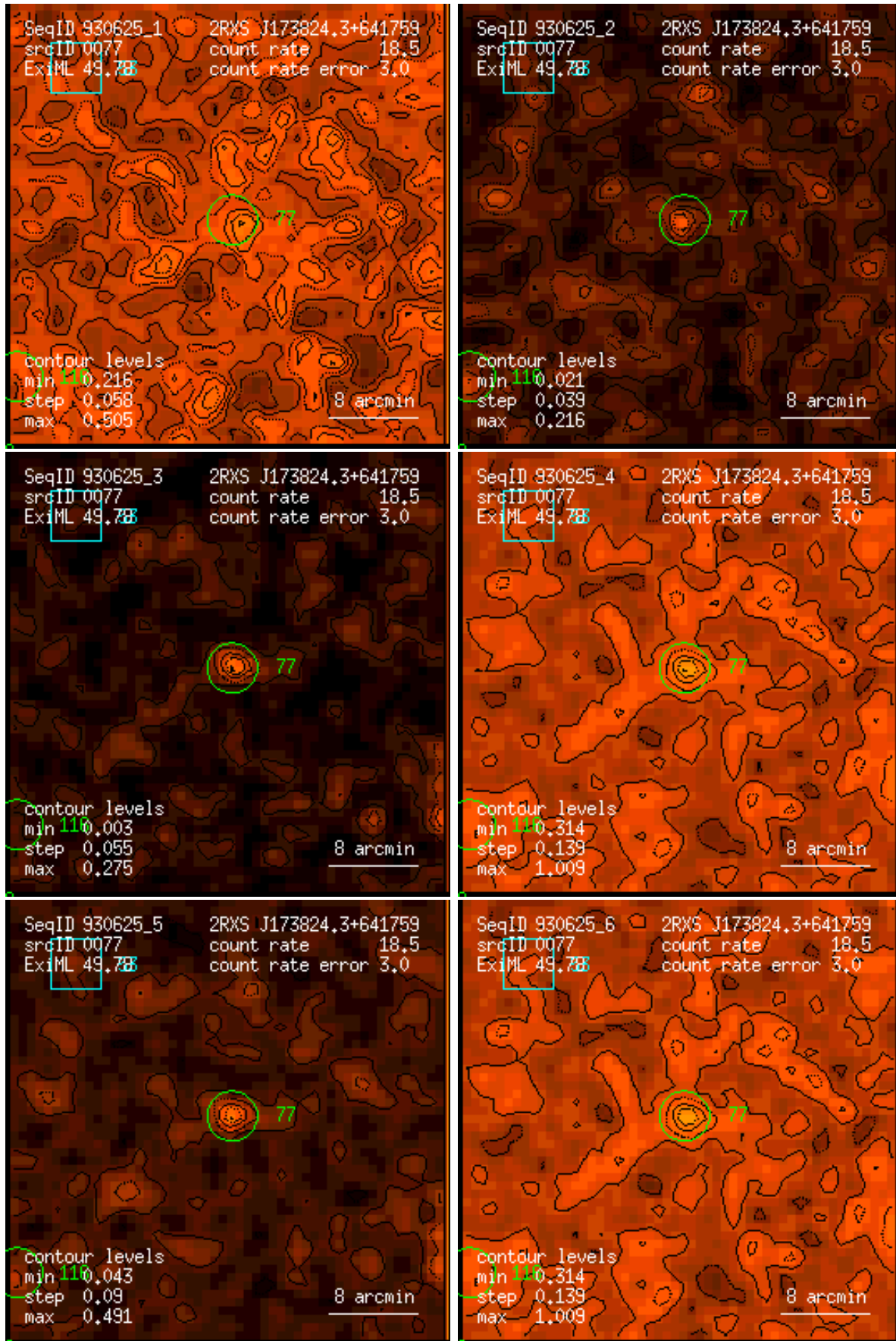
Figure 77: RASS 930625: detection 0077: band rate images, Gaussian filter: (1) PSPC channels 11 – 41, (2) 52 – 90, (3) 91 – 201, (4) 11 – 235, (5) 52 – 201, (6) 11 – 201. Broad band rates in counts/ks. Band rate contour levels in counts/ks/arcmin 2 .
