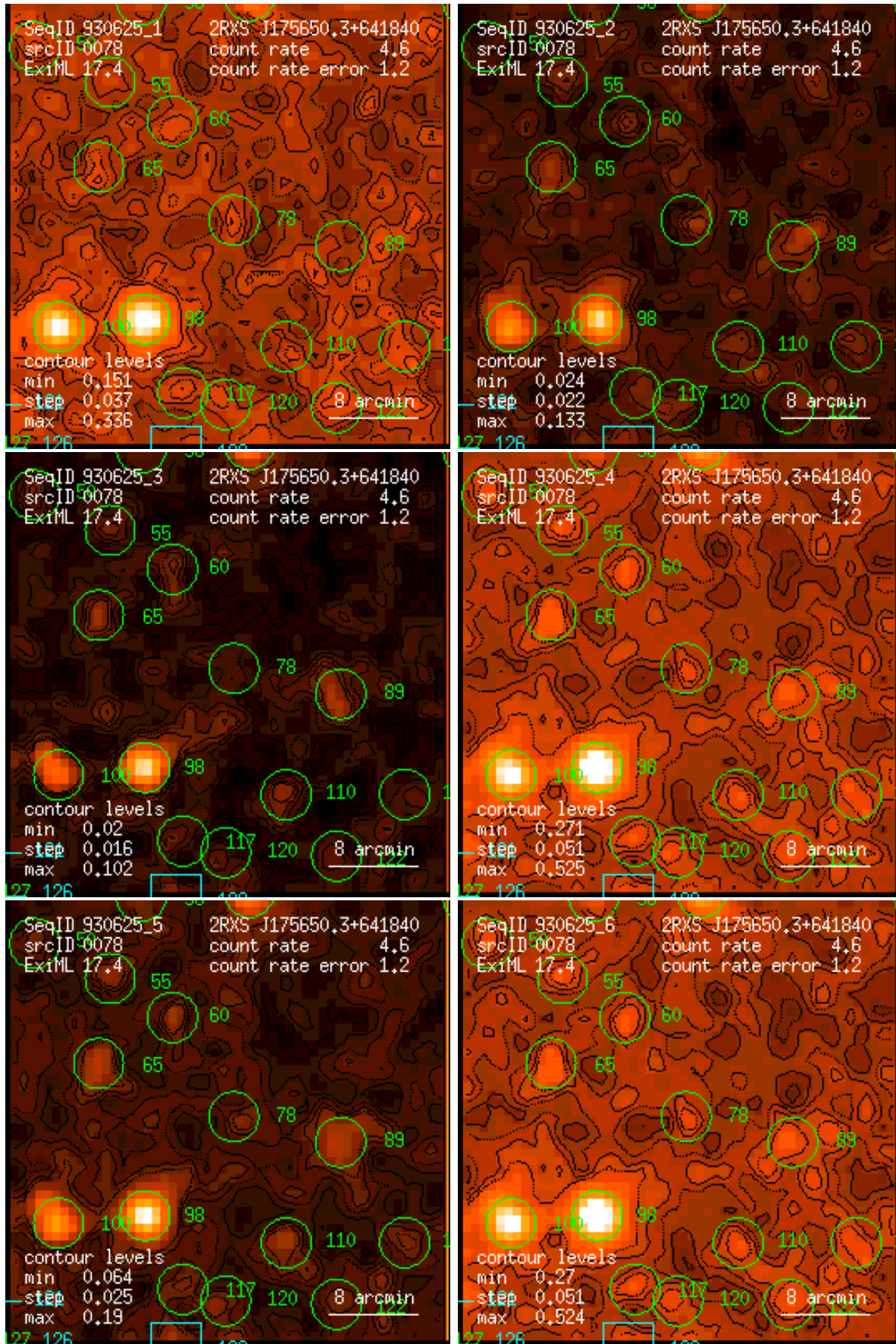
Figure 78: RASS 930625: detection 0078: band rate images, Gaussian filter: (1) PSPC channels 11 – 41, (2) 52 – 90, (3) 91 – 201, (4) 11 – 235, (5) 52 – 201, (6) 11 – 201. Broad band rates in counts/ks. Band rate contour levels in counts/ks/arcmin 2 .
