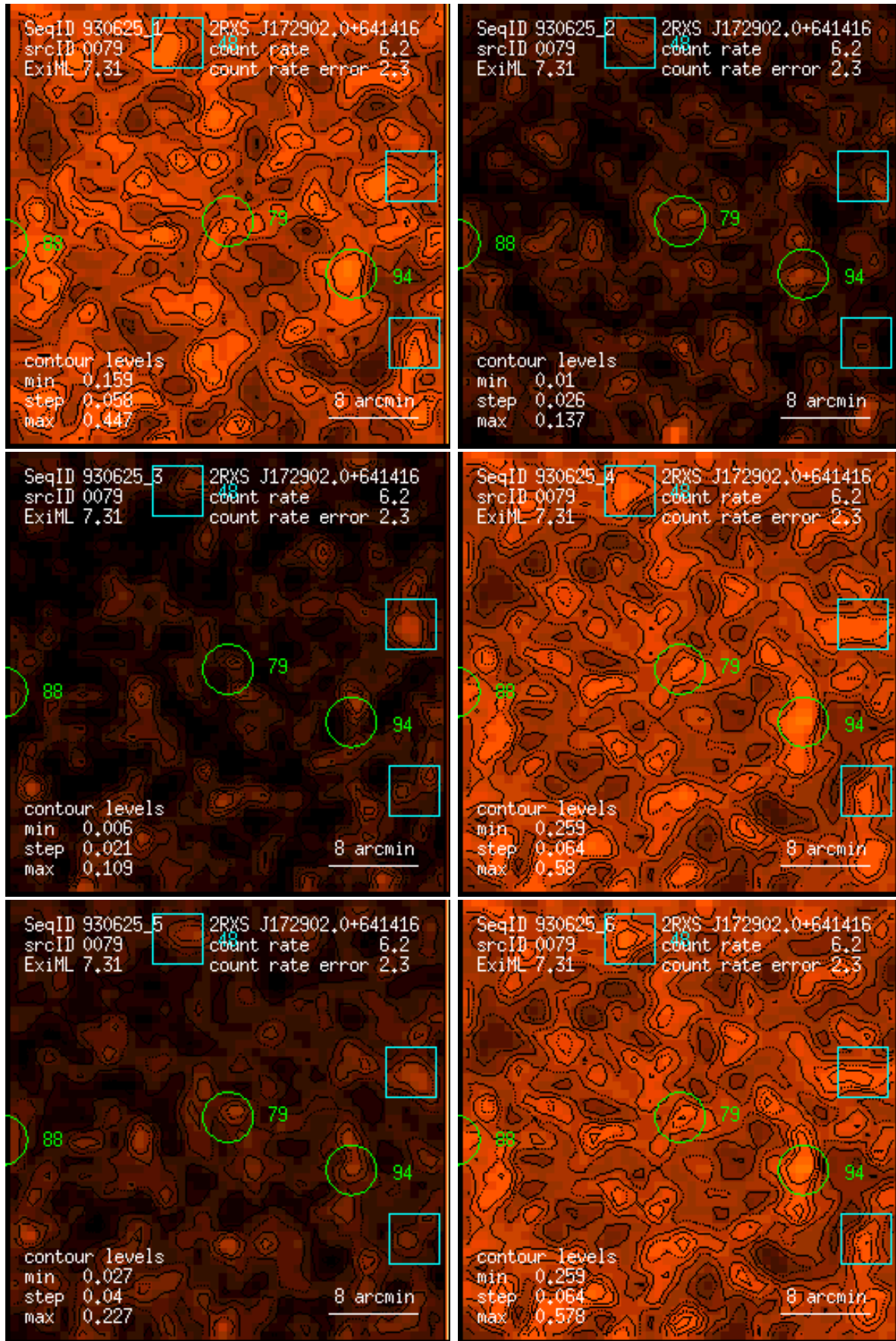
Figure 79: RASS 930625: detection 0079: band rate images, Gaussian filter: (1) PSPC channels 11 – 41, (2) 52 – 90, (3) 91 – 201, (4) 11 – 235, (5) 52 – 201, (6) 11 – 201. Broad band rates in counts/ks. Band rate contour levels in counts/ks/arcmin 2 .
