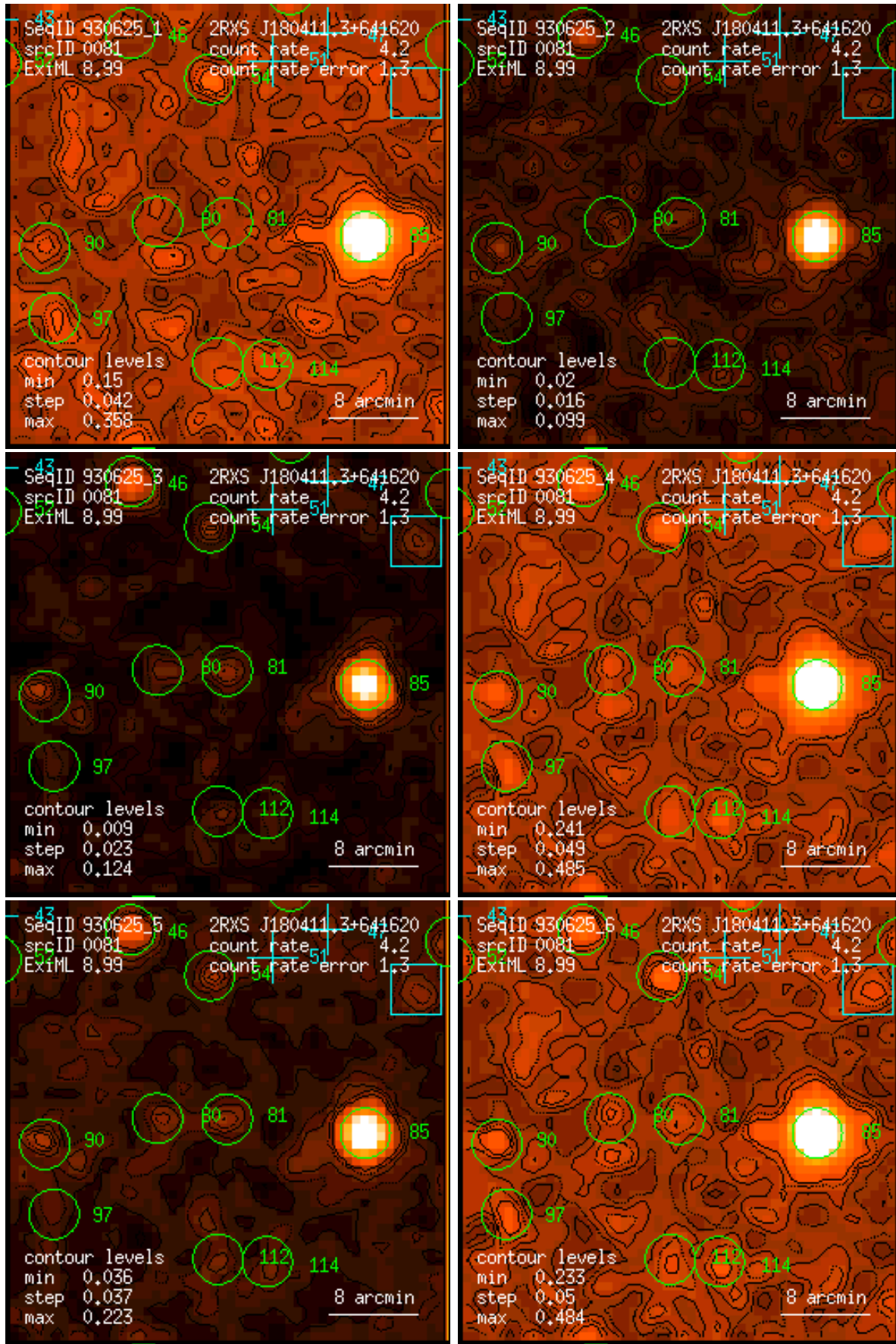
Figure 81: RASS 930625: detection 0081: band rate images, Gaussian filter: (1) PSPC channels 11 – 41, (2) 52 – 90, (3) 91 – 201, (4) 11 – 235, (5) 52 – 201, (6) 11 – 201. Broad band rates in counts/ks. Band rate contour levels in counts/ks/arcmin 2 .
