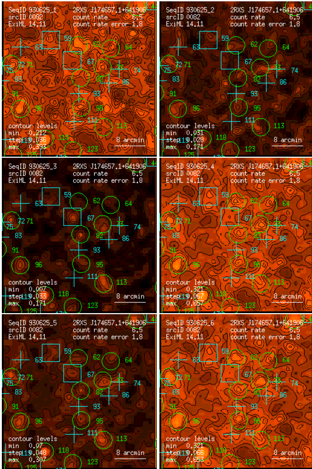
Figure 82: RASS 930625: detection 0082: band rate images, Gaussian filter: (1) PSPC channels 11 – 41, (2) 52 – 90, (3) 91 – 201, (4) 11 – 235, (5) 52 – 201, (6) 11 – 201. Broad band rates in counts/ks. Band rate contour levels in counts/ks/arcmin 2 .
