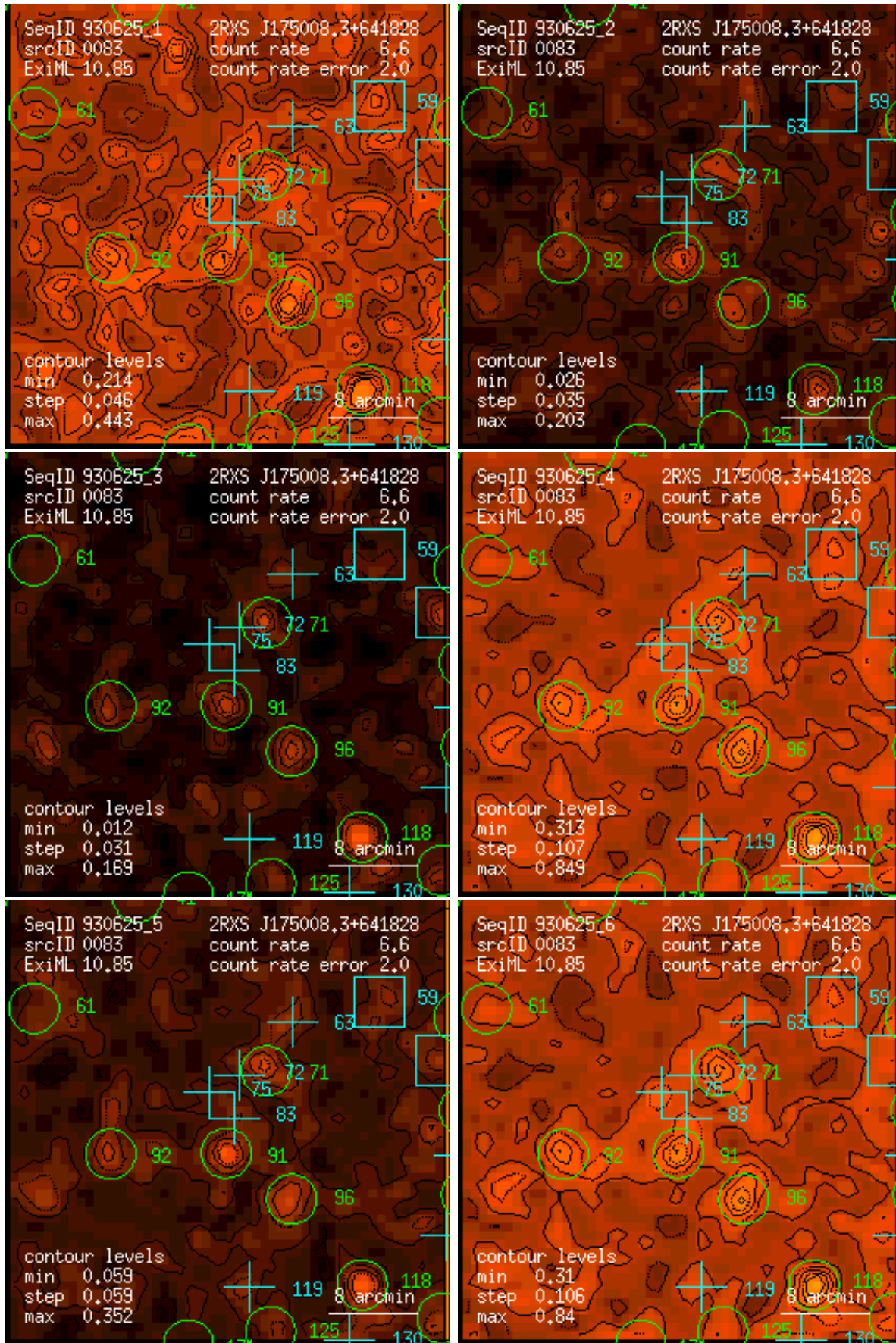
Figure 83: RASS 930625: detection 0083: band rate images, Gaussian filter: (1) PSPC channels 11 – 41, (2) 52 – 90, (3) 91 – 201, (4) 11 – 235, (5) 52 – 201, (6) 11 – 201. Broad band rates in counts/ks. Band rate contour levels in counts/ks/arcmin 2 .
