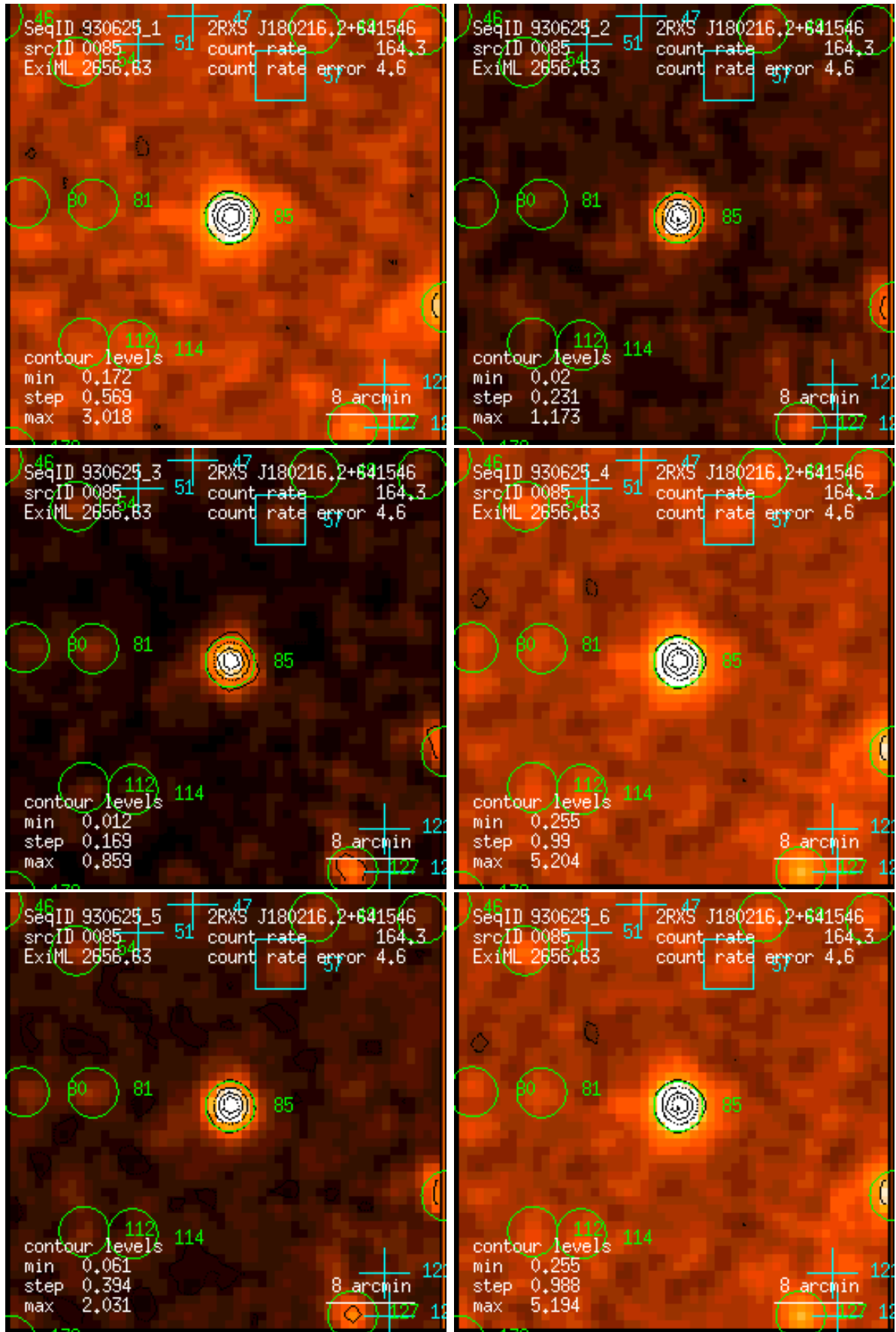
Figure 85: RASS 930625: detection 0085: band rate images, Gaussian filter: (1) PSPC channels 11 – 41, (2) 52 – 90, (3) 91 – 201, (4) 11 – 235, (5) 52 – 201, (6) 11 – 201. Broad band rates in counts/ks. Band rate contour levels in counts/ks/arcmin 2 .
