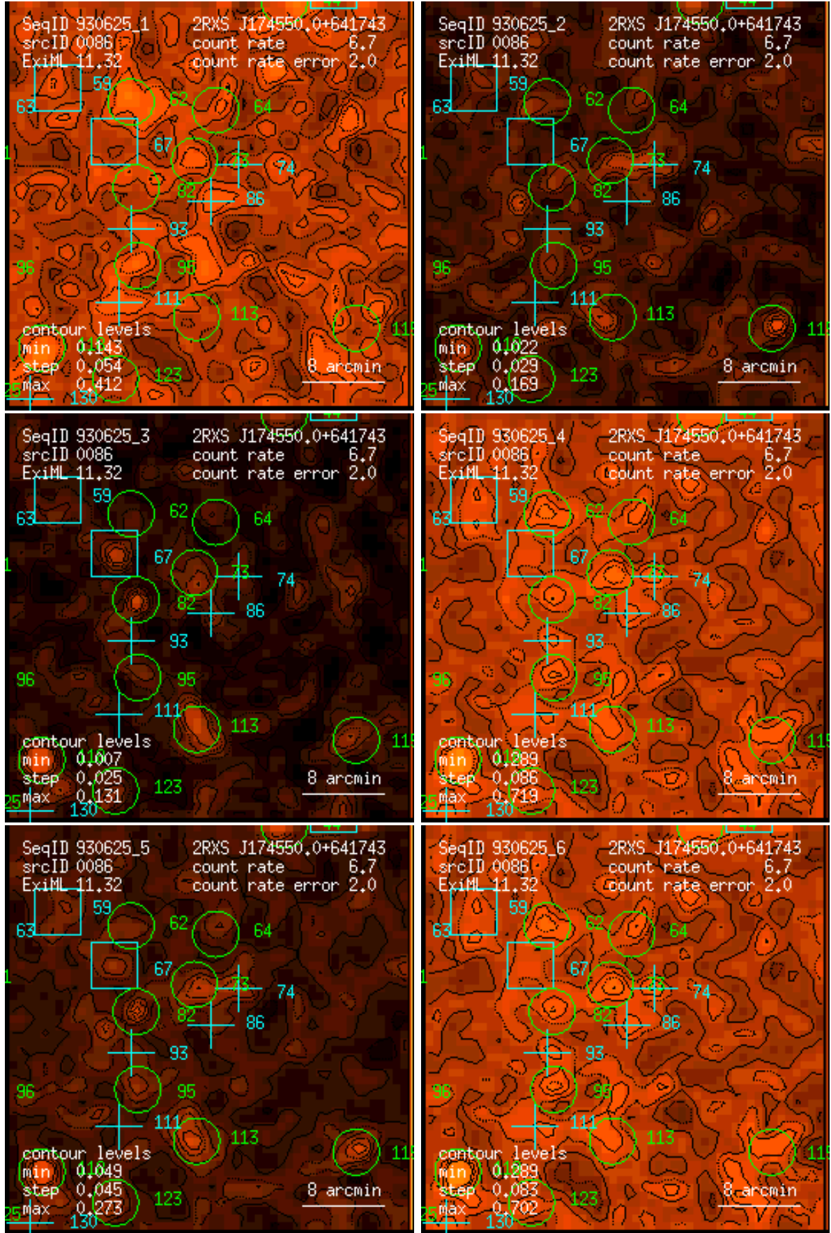
Figure 86: RASS 930625: detection 0086: band rate images, Gaussian filter: (1) PSPC channels 11 – 41, (2) 52 – 90, (3) 91 – 201, (4) 11 – 235, (5) 52 – 201, (6) 11 – 201. Broad band rates in counts/ks. Band rate contour levels in counts/ks/arcmin 2 .
