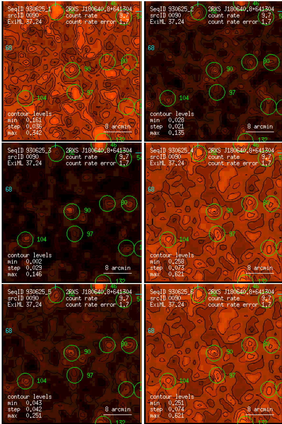
Figure 90: RASS 930625: detection 0090: band rate images, Gaussian filter: (1) PSPC channels 11 – 41, (2) 52 – 90, (3) 91 – 201, (4) 11 – 235, (5) 52 – 201, (6) 11 – 201. Broad band rates in counts/ks. Band rate contour levels in counts/ks/arcmin 2 .
