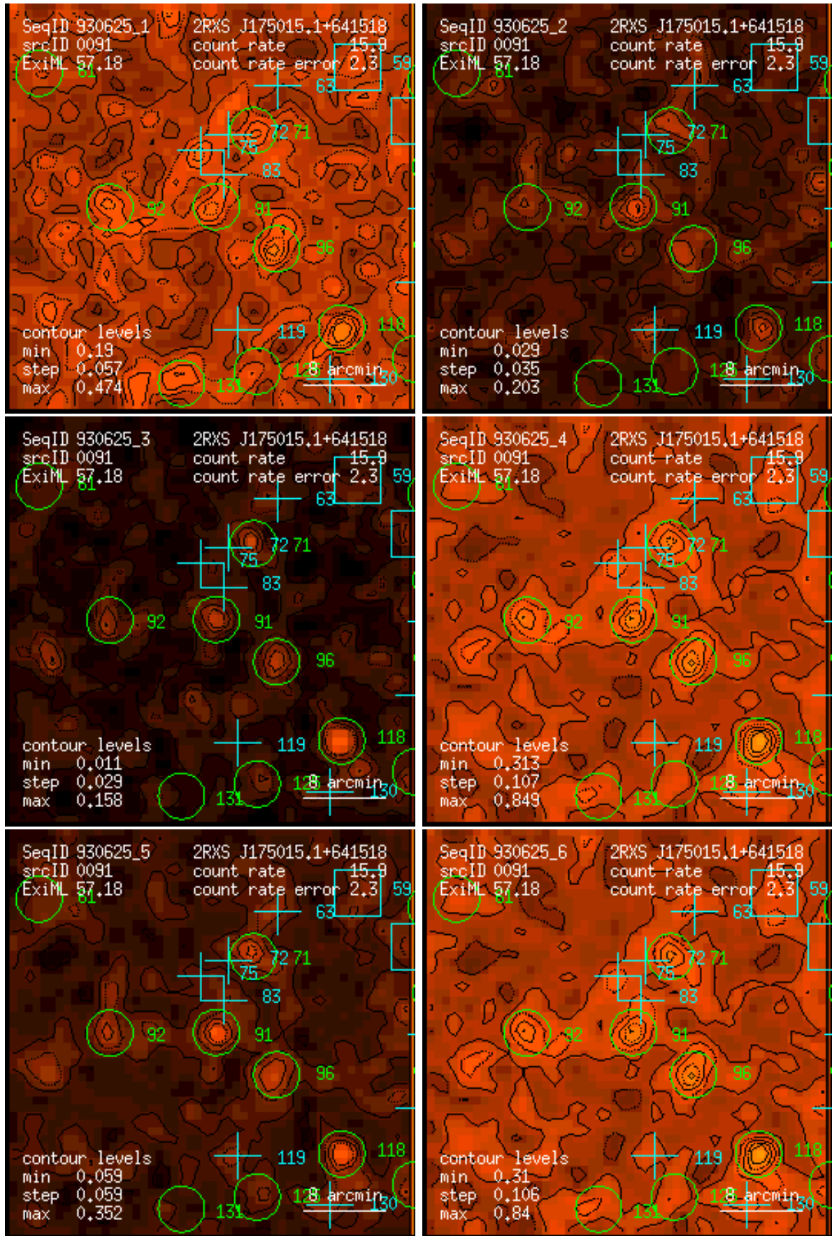
Figure 91: RASS 930625: detection 0091: band rate images, Gaussian filter: (1) PSPC channels 11 – 41, (2) 52 – 90, (3) 91 – 201, (4) 11 – 235, (5) 52 – 201, (6) 11 – 201. Broad band rates in counts/ks. Band rate contour levels in counts/ks/arcmin 2 .
