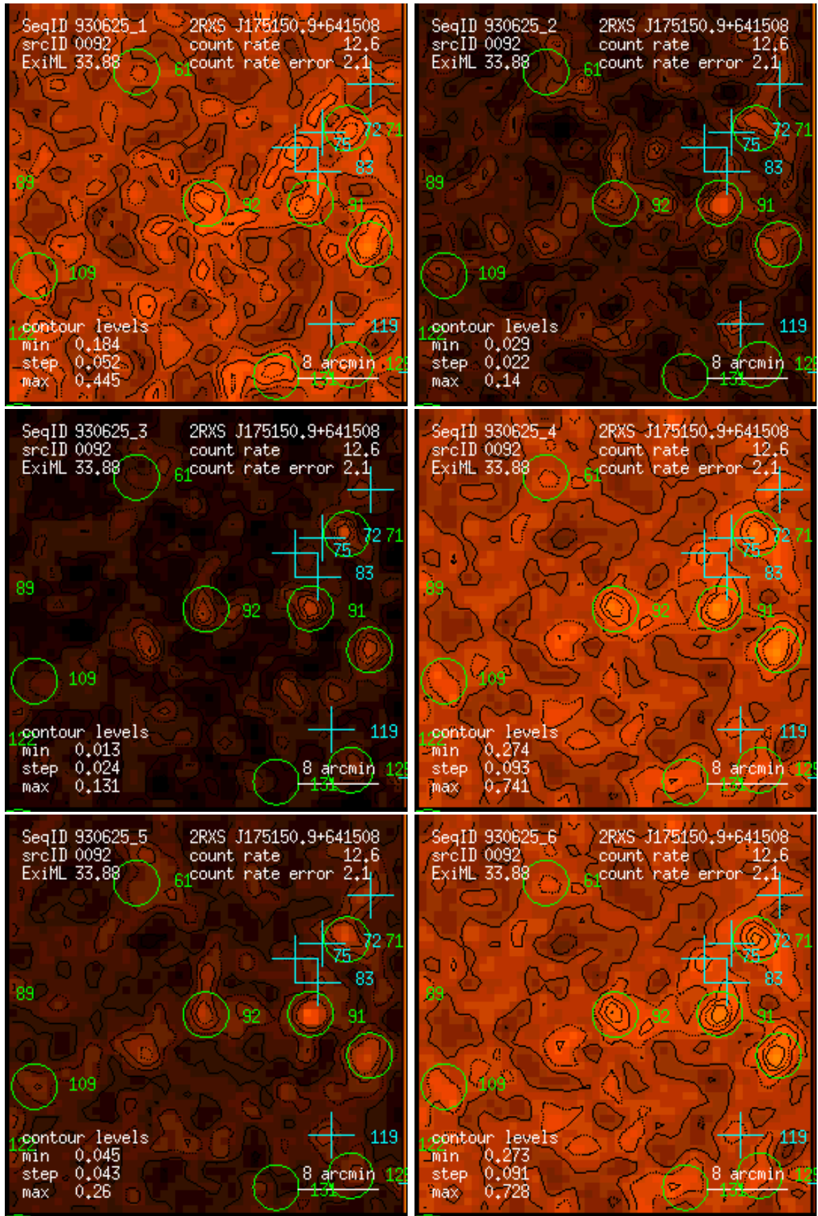
Figure 92: RASS 930625: detection 0092: band rate images, Gaussian filter: (1) PSPC channels 11 – 41, (2) 52 – 90, (3) 91 – 201, (4) 11 – 235, (5) 52 – 201, (6) 11 – 201. Broad band rates in counts/ks. Band rate contour levels in counts/ks/arcmin 2 .
