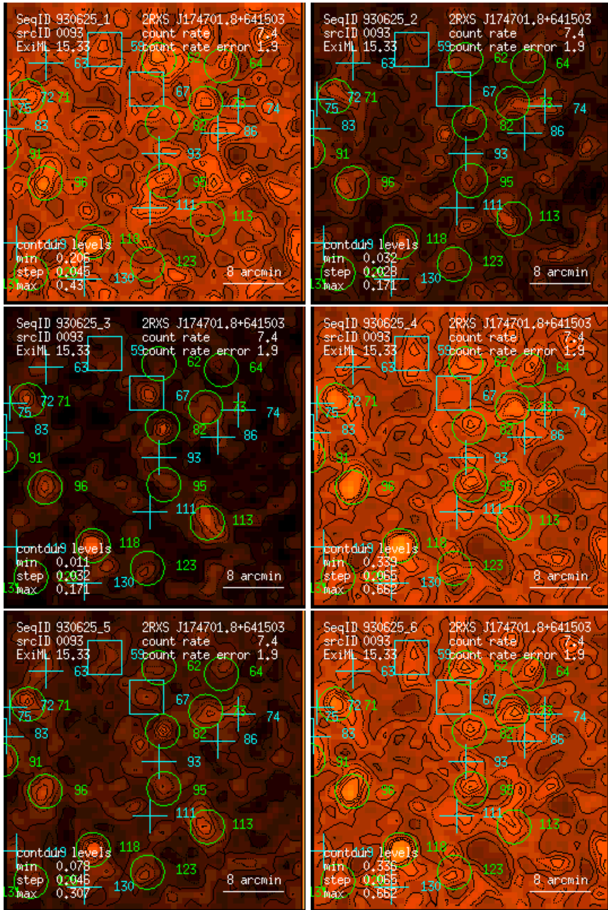
Figure 93: RASS 930625: detection 0093: band rate images, Gaussian filter: (1) PSPC channels 11 – 41, (2) 52 – 90, (3) 91 – 201, (4) 11 – 235, (5) 52 – 201, (6) 11 – 201. Broad band rates in counts/ks. Band rate contour levels in counts/ks/arcmin 2 .
