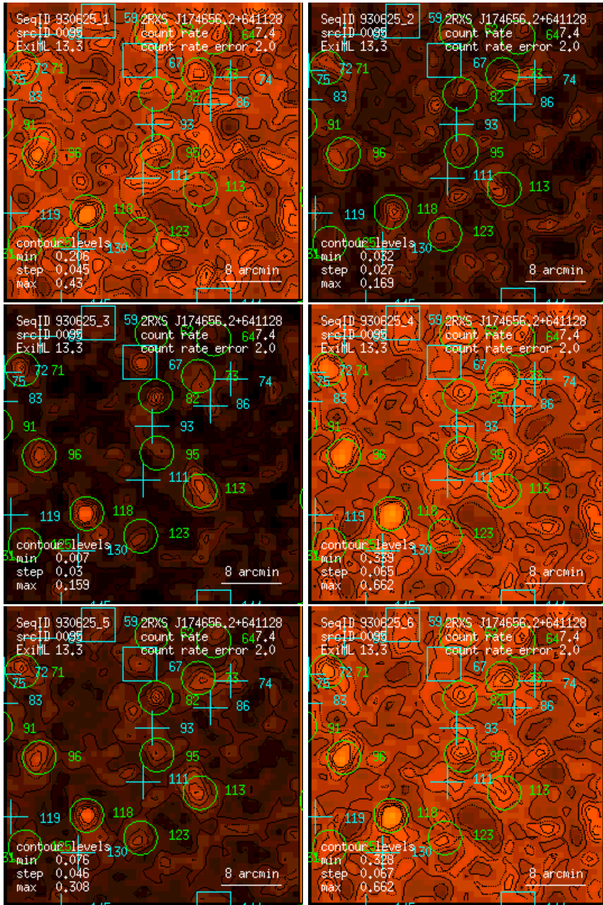
Figure 95: RASS 930625: detection 0095: band rate images, Gaussian filter: (1) PSPC channels 11 – 41, (2) 52 – 90, (3) 91 – 201, (4) 11 – 235, (5) 52 – 201, (6) 11 – 201. Broad band rates in counts/ks. Band rate contour levels in counts/ks/arcmin 2 .
