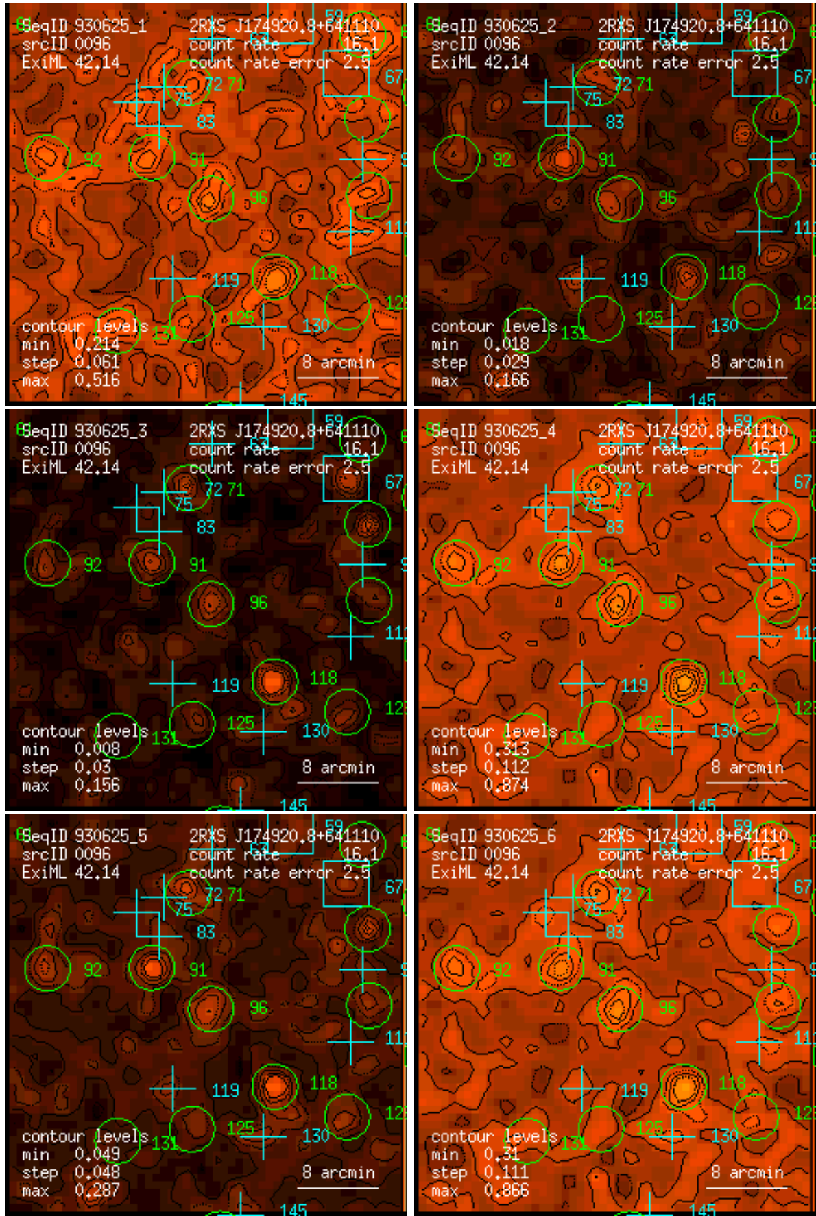
Figure 96: RASS 930625: detection 0096: band rate images, Gaussian filter: (1) PSPC channels 11 – 41, (2) 52 – 90, (3) 91 – 201, (4) 11 – 235, (5) 52 – 201, (6) 11 – 201. Broad band rates in counts/ks. Band rate contour levels in counts/ks/arcmin 2 .
