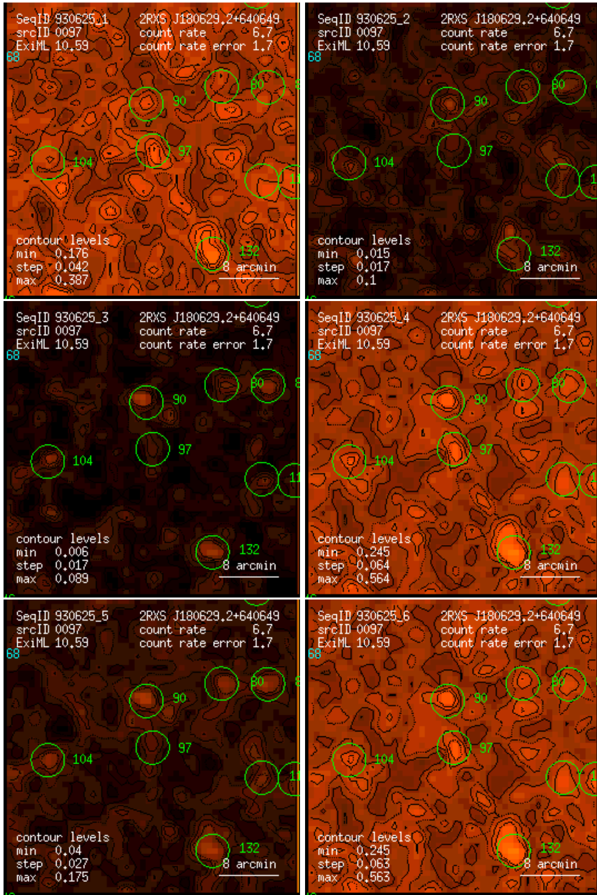
Figure 97: RASS 930625: detection 0097: band rate images, Gaussian filter: (1) PSPC channels 11 – 41, (2) 52 – 90, (3) 91 – 201, (4) 11 – 235, (5) 52 – 201, (6) 11 – 201. Broad band rates in counts/ks. Band rate contour levels in counts/ks/arcmin 2 .
