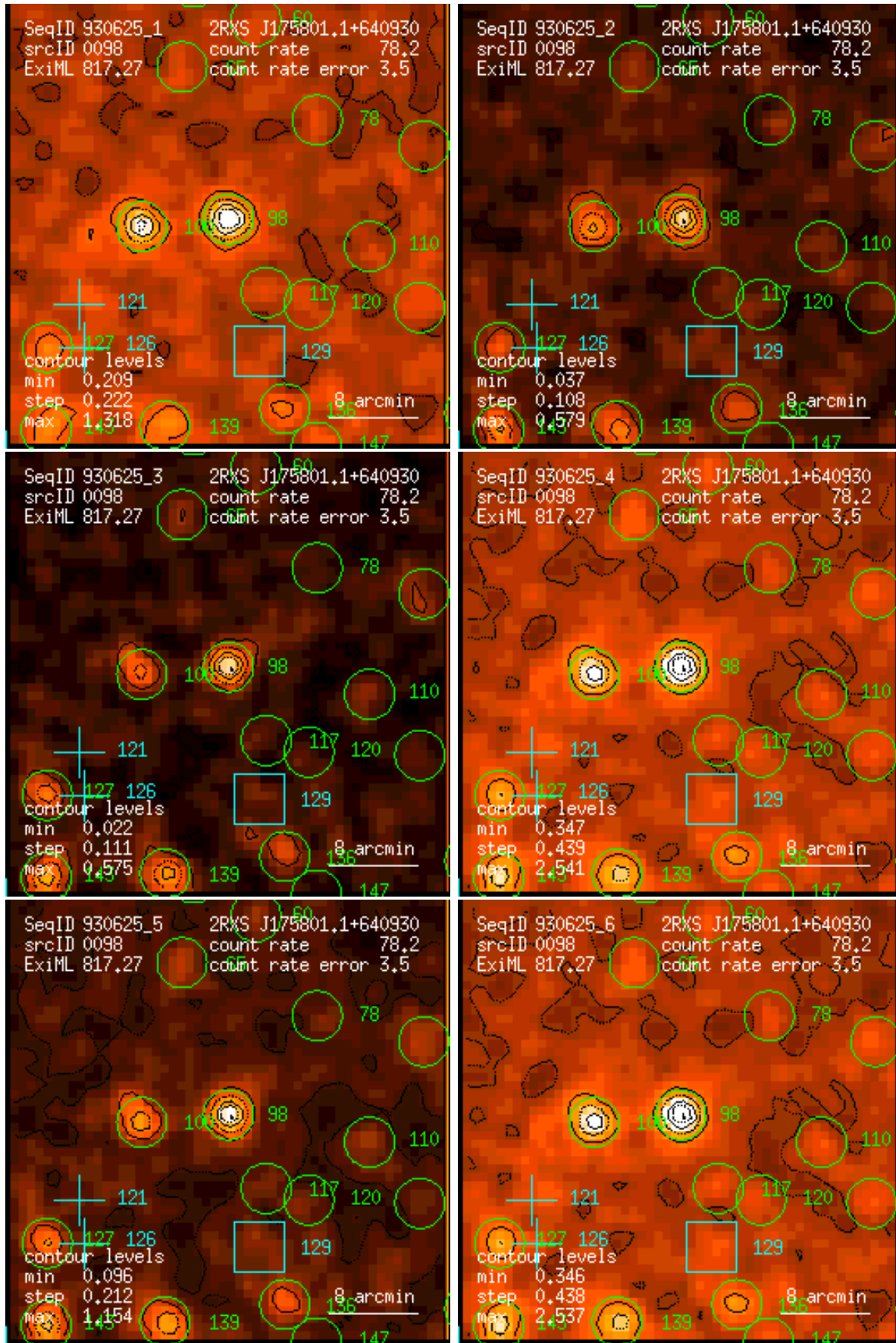
Figure 98: RASS 930625: detection 0098: band rate images, Gaussian filter: (1) PSPC channels 11 – 41, (2) 52 – 90, (3) 91 – 201, (4) 11 – 235, (5) 52 – 201, (6) 11 – 201. Broad band rates in counts/ks. Band rate contour levels in counts/ks/arcmin 2 .
