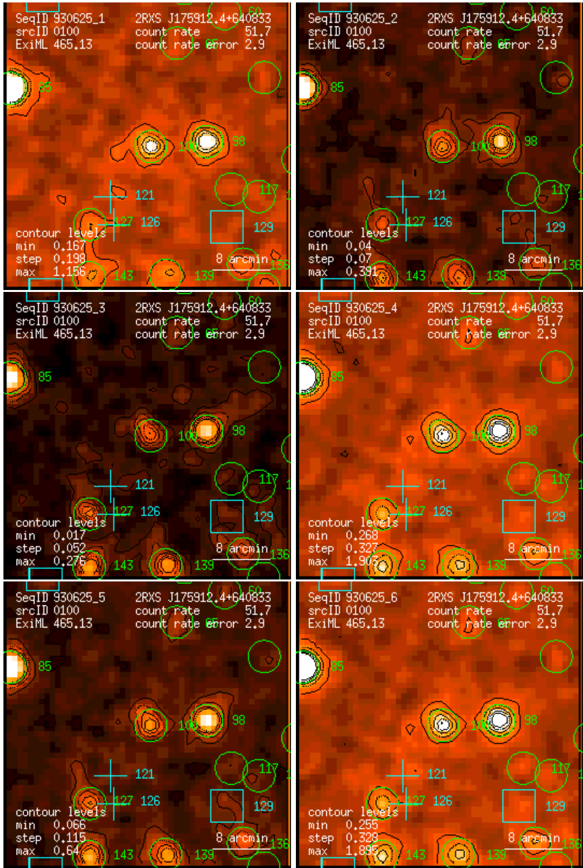
Figure 100: RASS 930625: detection 0100: band rate images, Gaussian filter: (1) PSPC channels 11 – 41, (2) 52 – 90, (3) 91 – 201, (4) 11 – 235, (5) 52 – 201, (6) 11 – 201. Broad band rates in counts/ks. Band rate contour levels in counts/ks/arcmin 2 .
