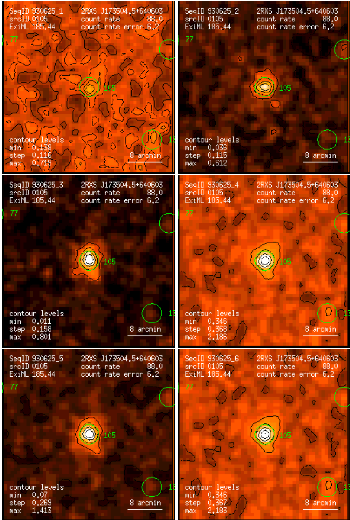
Figure 105: RASS 930625: detection 0105: band rate images, Gaussian filter: (1) PSPC channels 11 – 41, (2) 52 – 90, (3) 91 – 201, (4) 11 – 235, (5) 52 – 201, (6) 11 – 201. Broad band rates in counts/ks. Band rate contour levels in counts/ks/arcmin 2 .
