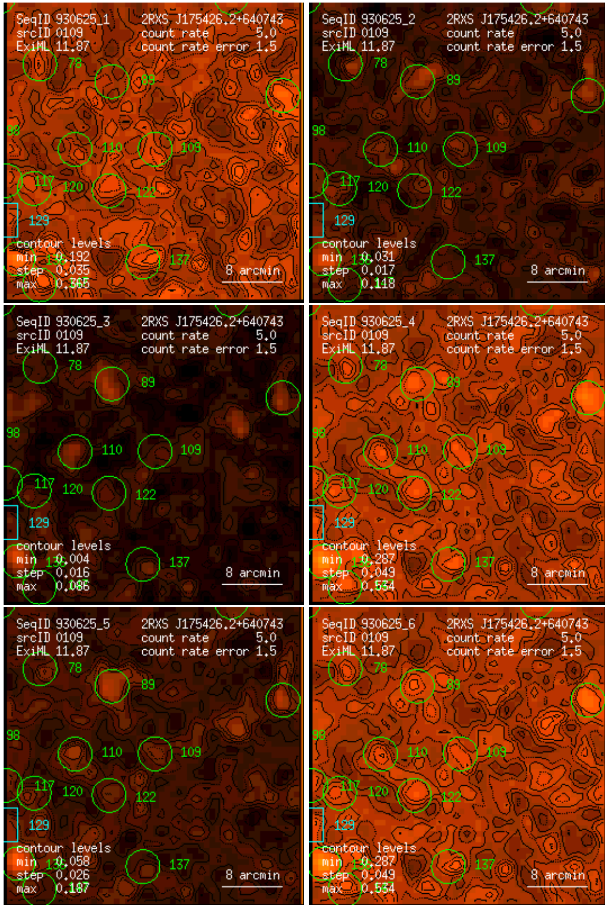
Figure 109: RASS 930625: detection 0109: band rate images, Gaussian filter: (1) PSPC channels 11 – 41, (2) 52 – 90, (3) 91 – 201, (4) 11 – 235, (5) 52 – 201, (6) 11 – 201. Broad band rates in counts/ks. Band rate contour levels in counts/ks/arcmin 2 .
