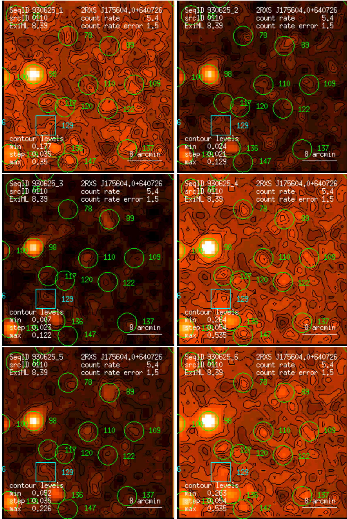
Figure 110: RASS 930625: detection 0110: band rate images, Gaussian filter: (1) PSPC channels 11 – 41, (2) 52 – 90, (3) 91 – 201, (4) 11 – 235, (5) 52 – 201, (6) 11 – 201. Broad band rates in counts/ks. Band rate contour levels in counts/ks/arcmin 2 .
