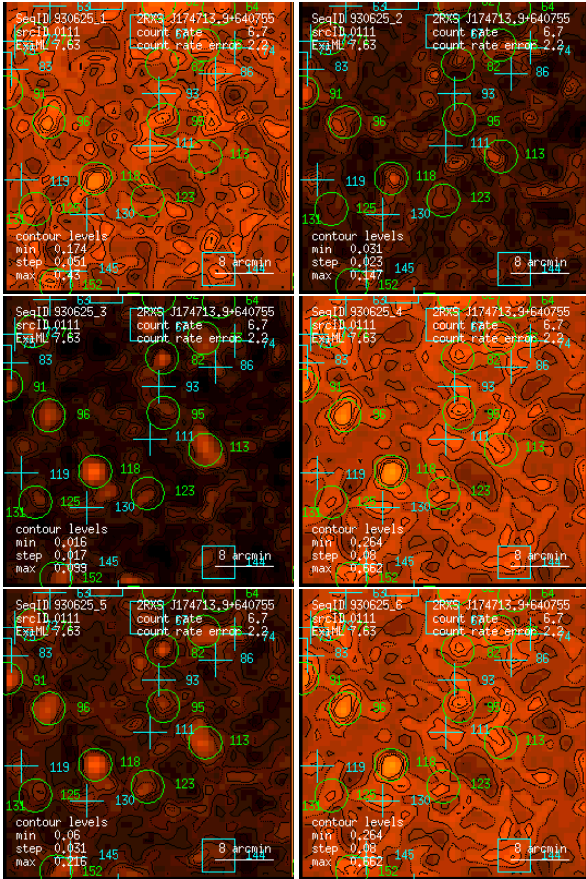
Figure 111: RASS 930625: detection 0111: band rate images, Gaussian filter: (1) PSPC channels 11 – 41, (2) 52 – 90, (3) 91 – 201, (4) 11 – 235, (5) 52 – 201, (6) 11 – 201. Broad band rates in counts/ks. Band rate contour levels in counts/ks/arcmin 2 .
