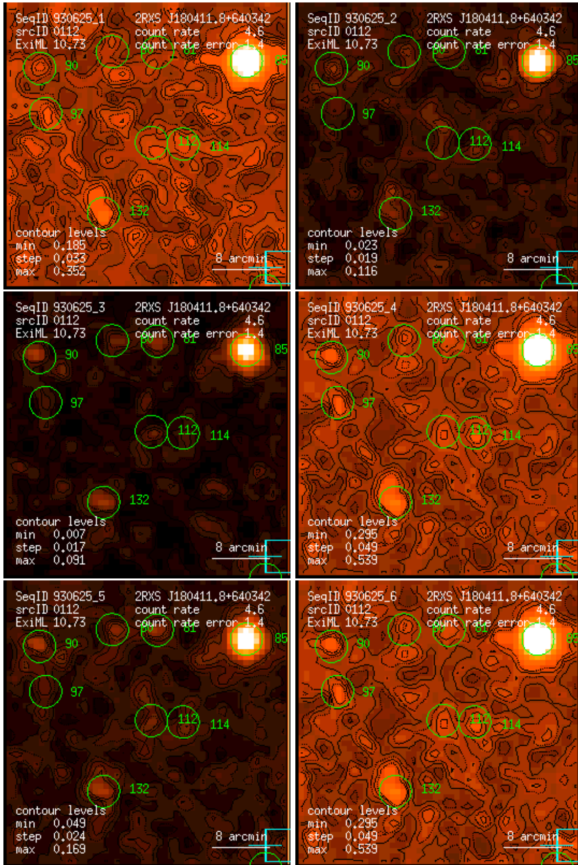
Figure 112: RASS 930625: detection 0112: band rate images, Gaussian filter: (1) PSPC channels 11 – 41, (2) 52 – 90, (3) 91 – 201, (4) 11 – 235, (5) 52 – 201, (6) 11 – 201. Broad band rates in counts/ks. Band rate contour levels in counts/ks/arcmin 2 .
