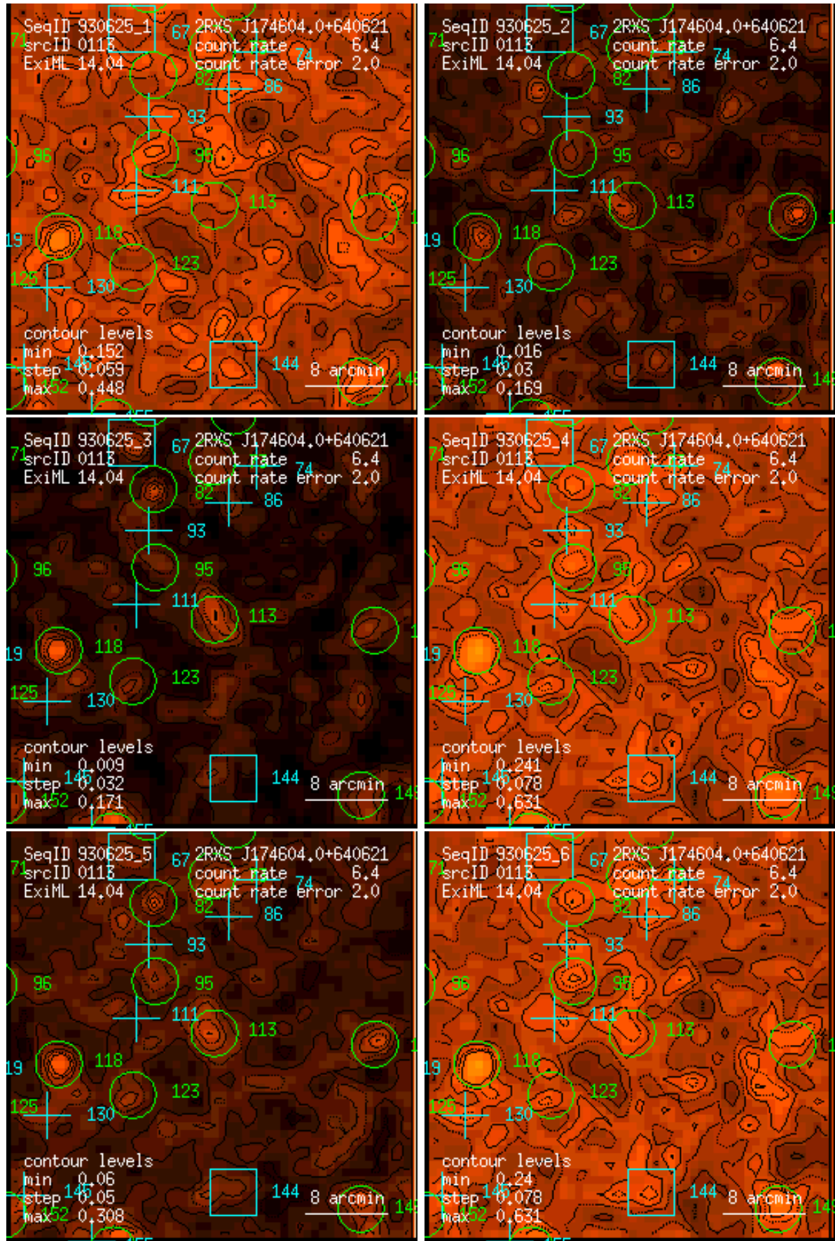
Figure 113: RASS 930625: detection 0113: band rate images, Gaussian filter: (1) PSPC channels 11 – 41, (2) 52 – 90, (3) 91 – 201, (4) 11 – 235, (5) 52 – 201, (6) 11 – 201. Broad band rates in counts/ks. Band rate contour levels in counts/ks/arcmin 2 .
