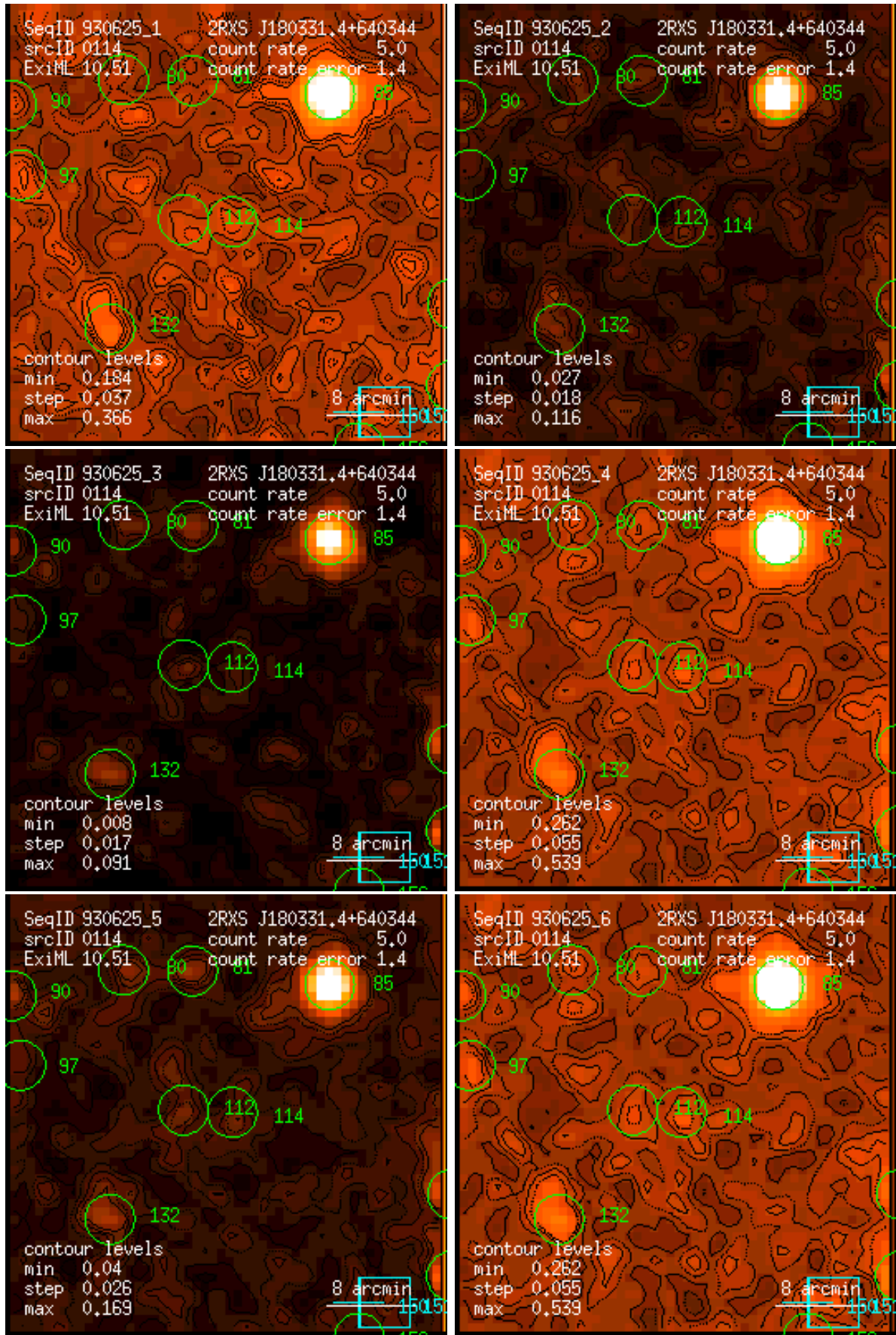
Figure 114: RASS 930625: detection 0114: band rate images, Gaussian filter: (1) PSPC channels 11 – 41, (2) 52 – 90, (3) 91 – 201, (4) 11 – 235, (5) 52 – 201, (6) 11 – 201. Broad band rates in counts/ks. Band rate contour levels in counts/ks/arcmin 2 .
