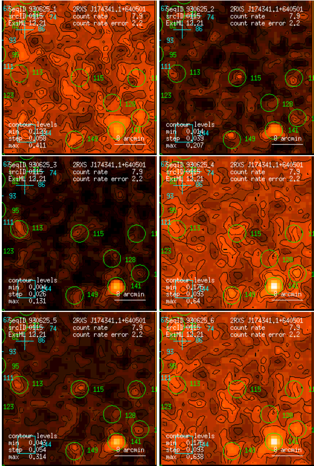
Figure 115: RASS 930625: detection 0115: band rate images, Gaussian filter: (1) PSPC channels 11 – 41, (2) 52 – 90, (3) 91 – 201, (4) 11 – 235, (5) 52 – 201, (6) 11 – 201. Broad band rates in counts/ks. Band rate contour levels in counts/ks/arcmin 2 .
